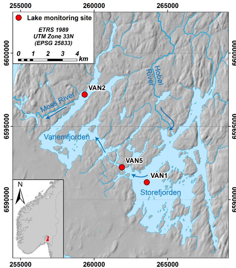
Figure 1. Lake Vansjø in southeast Norway, showing the two main basins: the larger eastern basin (Storefjorden) and Vanemfjorden (the study basin), which has its outlet at Moss River. The two basins are connected by a narrow channel. The largest tributary to Lake Vansjø is the Hobøl River. Main NIVA monitoring sites are shown and arrows show the dominant flow directions. Here, we use data from VAN2. Hillshade ©Kartverket ( https://www.kartverket.no/ , last accessed 09/05/2022), hydrologic data ©NVE ( https://www.nve.no/english/ , last accessed 09/05/2022).
