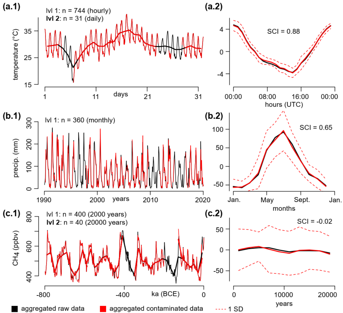
Fig. 6. Aggregation of the temperature (panel a), precipitation (panel b) and methane (panel c) in two consecutive levels: 1 (thin lines) and 2 (bold lines). Only the first level of aggregated precipitation is shown for clarity. Black and red colors are associated with the raw and contaminated datasets, respectively. The mean cycles of the second level of aggregation are shown in the second column, with their SCI displayed (the raw and contaminated versions share similar values).
