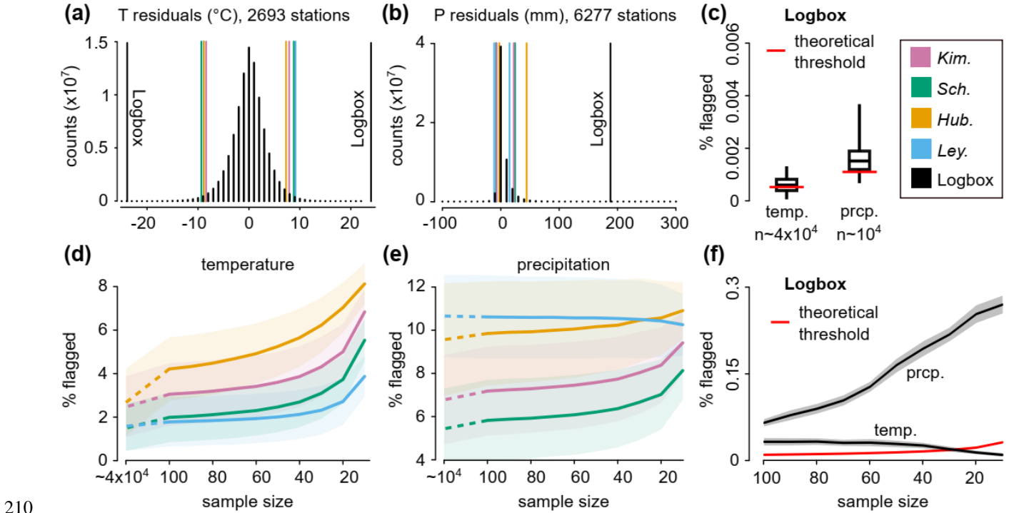
Fig. 2. Comparison between five outlier detection methods performed on two sets of residuals (temperature and precipitation) obtained from weather stations with daily measurements over at least 100 years. The two histograms (panels a and b ) represent aggregated residuals from all stations (for visualization purpose only) and show counts with at least 100 daily occurrences, with the median of the lower/upper threshold displayed for each method. For the methods Kim. (Kimber, 1990), Sch. (Schwertman et al., 2004), Hub. (Hubert & Vandervieren, 2008) and Ley. (Leys et al., 2013), the mean percentage ( \pm 1 SD) of flagged data is shown for sample sizes varying from 10 to 100, and for all available points per station ( n \sim 4 \times 10^4 for the temperature and n \sim 10^4 for the precipitation, panels d and e ). For Logbox (panels c and f ), this percentage is calculated by pooling all points, and the variability is estimated with a random resampling of stations (see method). The theoretical threshold is the expected percentage of erroneously flagged outliers ( p_{theo} = f(n) \times \frac{100}{n} = \frac{0.1}{\sqrt{n}} %).
