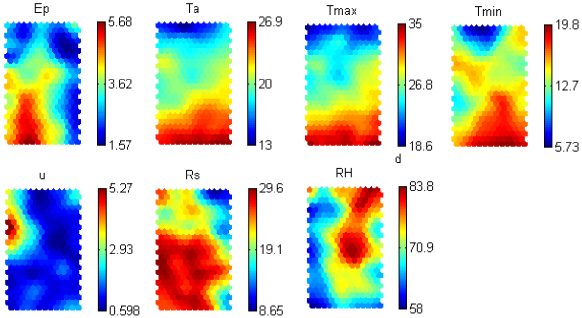
Figure 6: Kohonen Self-Organizing Map (K-SOM) visualization of pan evaporation and meteorological variables assessment ( T_a – daily mean temperature [°C], T_{max} – daily maximum temperature [°C], T_{min} – daily minimum temperature [°C], RH – relative humidity [%], R_s – global radiation [MJ m -2 d -1 ], u – wind speed [m s -1 ] and E_p - daily evaporation [mm d -1 ]). The bars indicate the intensity of the variables: the red colour is high importance, and the blue colour is low importance.
