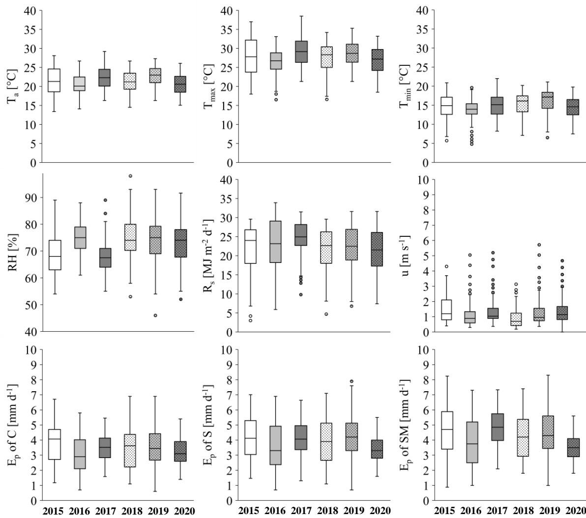
Figure 4: Box plot of meteorological parameters ( T_a – daily mean temperature [°C], T_{max} – daily maximum temperature [°C], T_{min} – daily minimum temperature [°C], RH – relative humidity [%], R_s – global radiation [ \text{MJ m}^{-2} \text{d}^{-1} ], u – wind speed [ \text{m s}^{-1} ] and daily evaporation of different pan treatments [ \text{mm d}^{-1} ] (C – control, S – Class A pan with sediment cover bottom, SM – Class A pan with submerged macrophyte) in 2015-2020 growing seasons (June-September). The lower and upper ends of the box indicate the 25 th and 75 th percentiles of the variances, respectively, while the horizontal bar within the box indicates the median. The two horizontal bars indicate the range that covers 90% of the variances. Outliers are indicated with circles.
