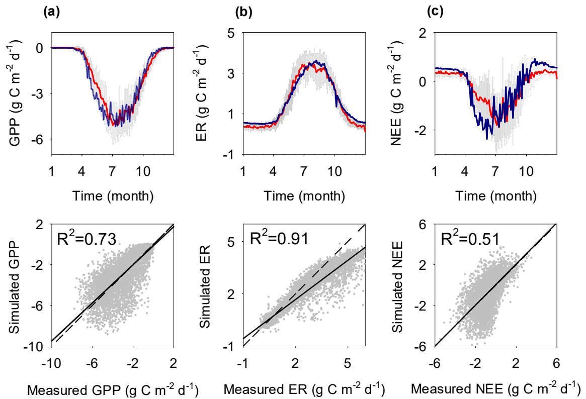
Figure 4: Mean annual seasonal cycle of simulated (blue line) and measured (red line \pm standard deviation as grey) ecosystem CO 2 fluxes, and scatter plots of simulated vs. measured fluxes: (a) gross primary production GPP, (b) ecosystem respiration ER, and (c) net ecosystem exchange NEE (1998-2018). Linear least-squares regressions (black lines) are fitted to the daily data. The 1:1 relationship is shown as a faint dotted line. R 2 denotes the coefficient of determination.
