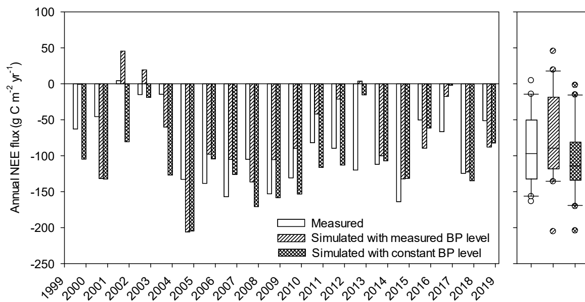
730 Figure 6: Simulated and measured annual NEE fluxes in the reference run (simulated with measured BP level) and the constant BP water level run (simulated with constant BP level).
