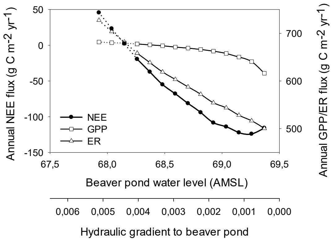
735 Figure 7: Sensitivity of annual mean NEE, GPP, ER to the varying beaver pond water level (thus lateral hydraulic gradient) for each 0.1 m bin of the pond level over 1998-2019. The constant BP water level ranged from 67.9 AMSL (a dry pond) to the highest possible water level, 69.37 AMSL (the average measured WTD at the peatland) when flow would reverse from the pond to the peatland. The solid line indicates the measured BP water table range. Note the sign of NEE follows the atmospheric convention, negative meaning uptake, and GPP and ER are both plotted as positive.
