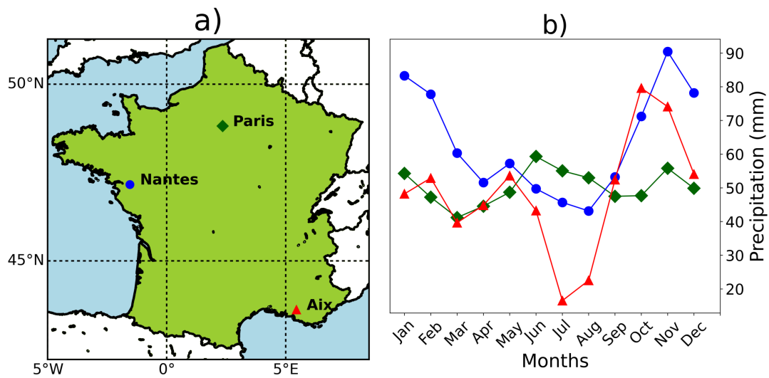
Figure 2. a) The three chosen cities/conurbations in mainland France, and b) their monthly cumulative precipitation climatology (using PDI , NDI and ADI daily datasets).
