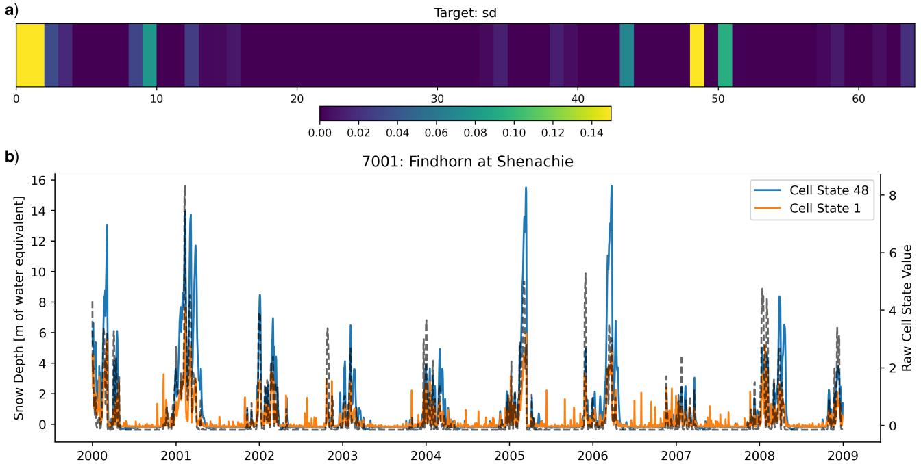
Figure 7. (a) We visualise the most informative weights where lighter colours means larger weights assigned to that cell state dimension by the linear probe. (b) The largest 2 dimensions, in terms of their assigned weight, from the above plot are then over-plotted on the snow depth target timeseries (grey dashed line), showing that they really do contain information about the winter snow signal, particularly Cell State 48 which varies very little in the summer months.
