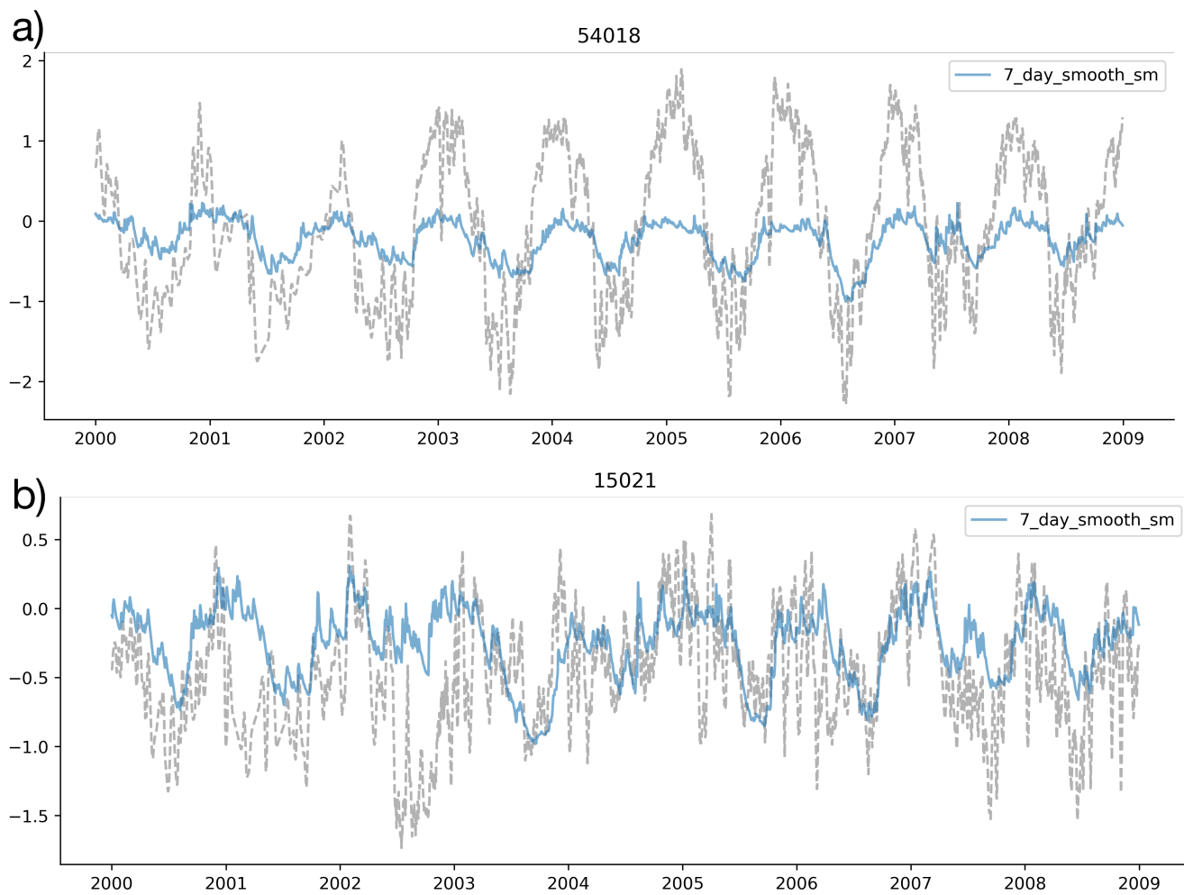
Figure B2. Time series of probe predictions (coloured lines) compared with the target variables (grey dotted lines). We show two catchments here, 54018 and 15021 for the ESA CCI Soil Moisture Products which is the same as Fig. 3
