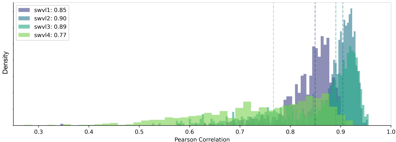
Figure 2. Histogram of catchment correlation scores for each soil water volume level: soil water volume level 1 (swvl1) contains soil moisture from depths of 0–7cm, soil water volume level 2 (swvl2) contains soil moisture from depths of 7–28cm, soil water volume level 3 (swvl3) contains soil moisture from depths of 28–100cm, soil water volume level 4 (swvl4) contains soil moisture from depths of 100–289cm.
