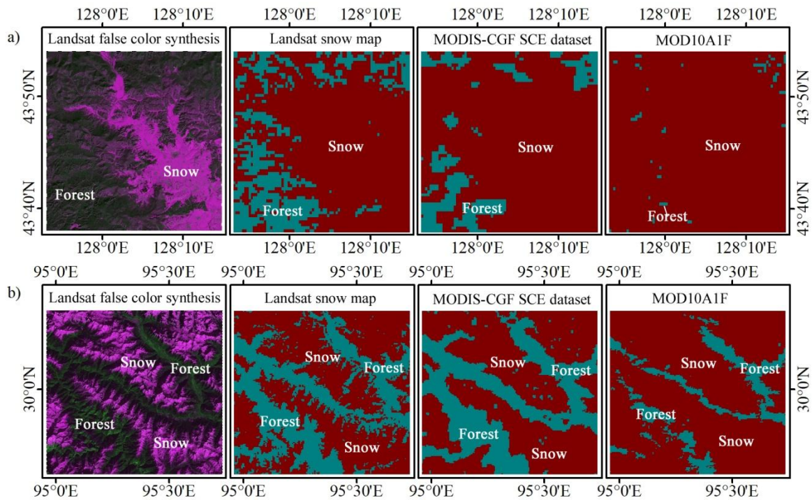
Figure 11: Intuitive improvements of CGF SCE in two representative forest areas: a) an example in Northeast China forest region; b) an example in Qinghai-Tibet Plateau forest region
