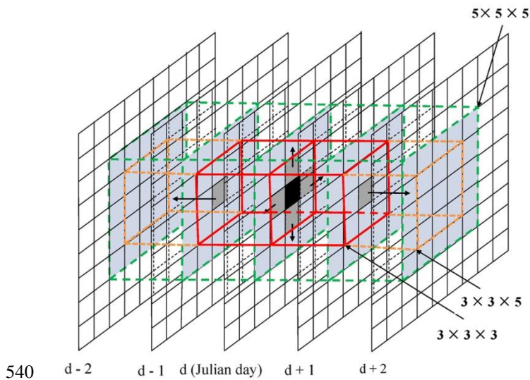
Figure 6: Diagram of the HMRF gap-filling process used in the study (Dark-grey represents high weight, and light-grey represents low weight)
