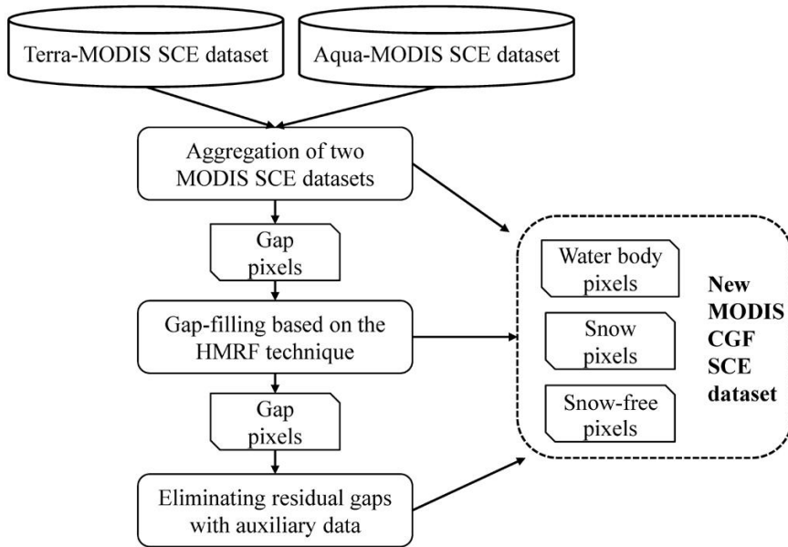
Figure 5: Flowchart of the new cloud-gap removing algorithm
