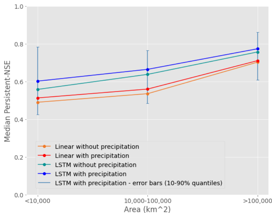
435 Figure 9. Persistent-NSE medians for three bins of watershed drainage area sizes. Number of gauges in the bins are 49, 54 and 42. Error bars are shown as the range of 10-90% quantiles in each bin. For a better visibility, they are only shown for the LSTM with precipitation model. For all four models the median of the largest bin is significantly different than the median of the middle bin and the smallest bin ( p\text{-val}<0.001 , based on Mood's median test), while the difference between medians of the two smaller bins is insignificant ( p\text{-val}>0.1 ).
