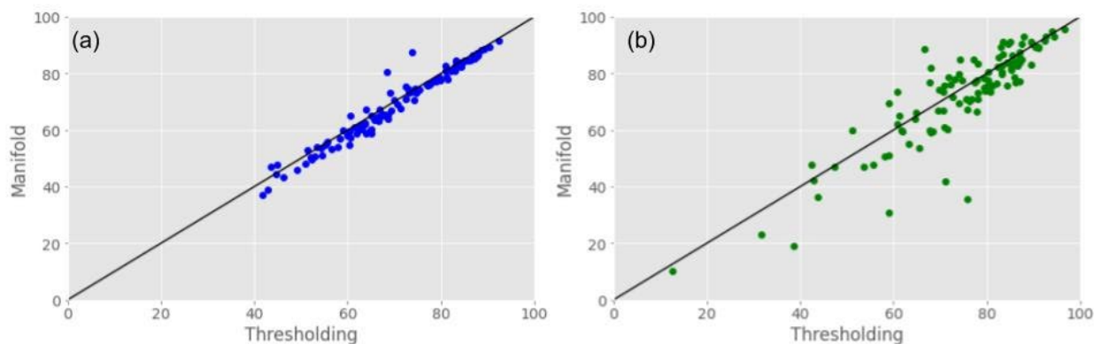
470 Figure 10. Comparison of the F1 metric between the Thresholding and Manifold inundation models for (a) 1-year cross-validation and (b) leave-extreme-out, based on data from 2016-2020, for 126 AOIs India and Bangladesh.
