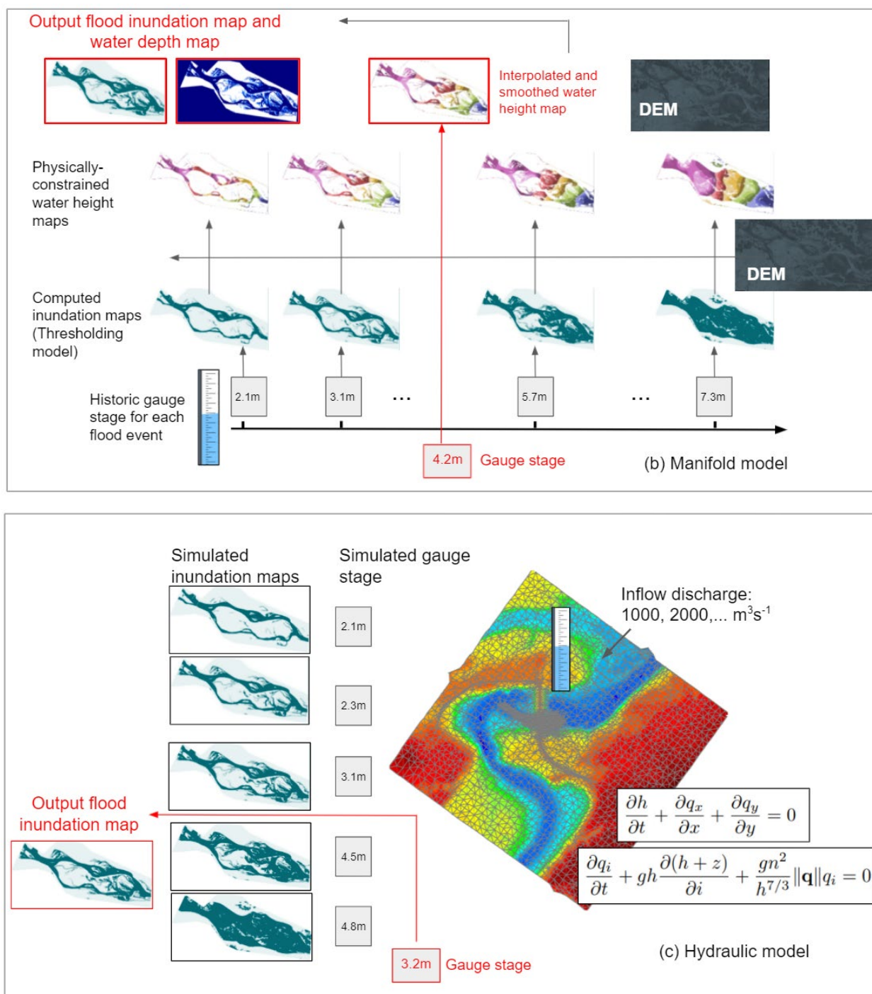
300 Figure 3. Schemes of the Thresholding (a), Manifold (b) and Hydraulic (c) flood inundation models
