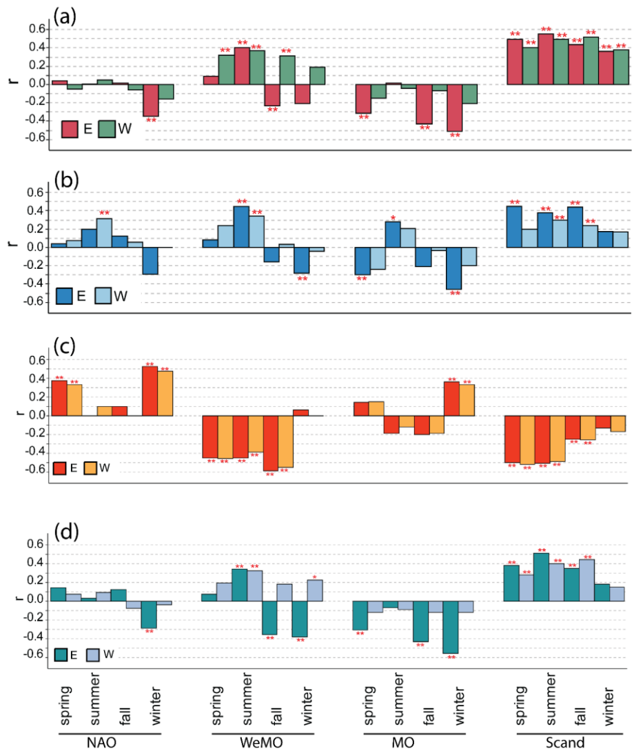
280 Figure 3: Estimated correlations between the teleconnection patterns and (a) RDI03 (b) Water discharge (c) Temperature (d) Precipitation. For (a), (c), and (d) the period considered is 1959-2018, whereas in (b) the period considered is 1976-2018. Water discharge for each cluster is the sum of each river's water discharge for whose the watershed belongs to either one of the cluster. Thus, Western discharge is the sum of the Aude, Agly and Tet water discharge and eastern discharge the sum of Herault, Orb and Tech water discharge
