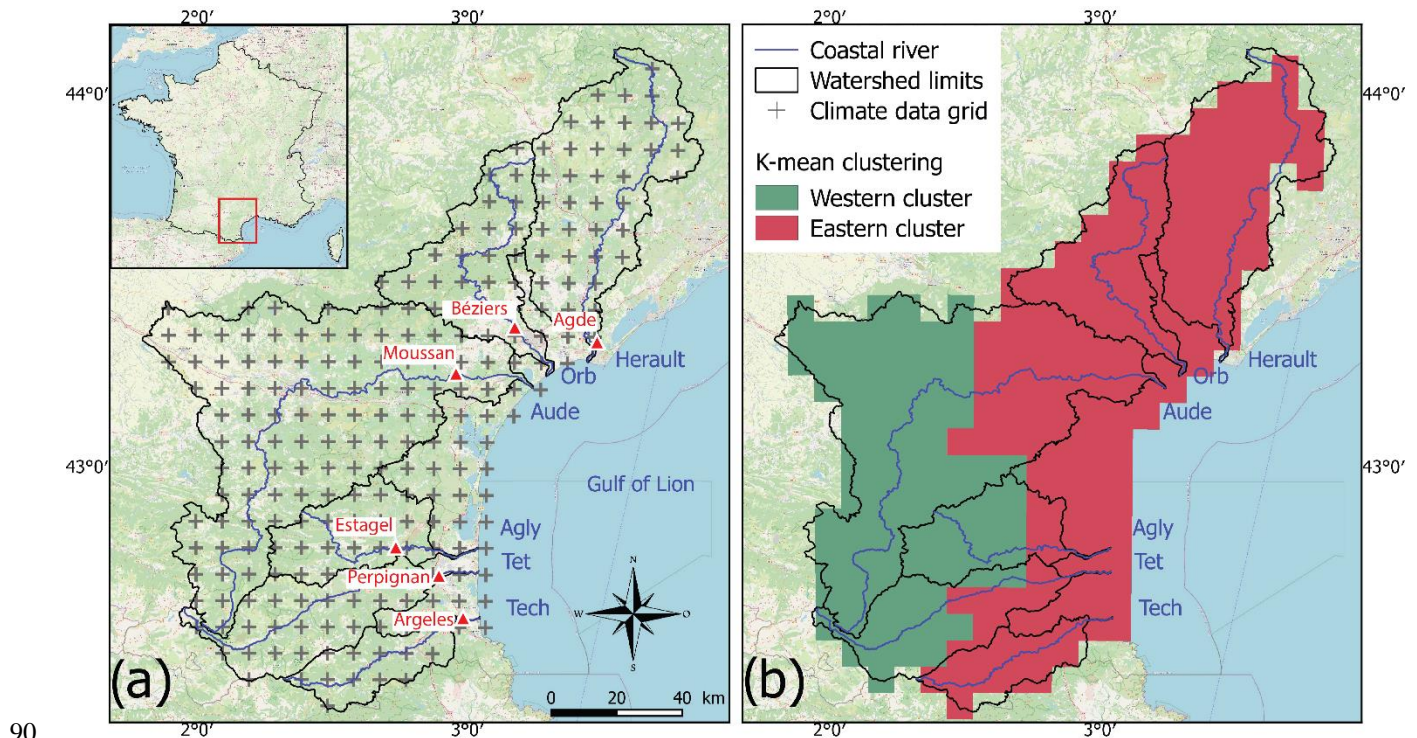
Figure 1 : Location and characteristics of the study area. a) Watersheds limits, rivers, and Safran grid with daily temperature and precipitation. Red triangles are the gauging stations used for historical evolution of the annual water discharge for each river b) Cluster distribution obtained by the k-mean method applied to RDI-03 data over the period 1959-2018. Map data: © OpenStreetMap contributors 2021. Distributed under the Open Data Commons Open Database License (ODbL) v1.0.
