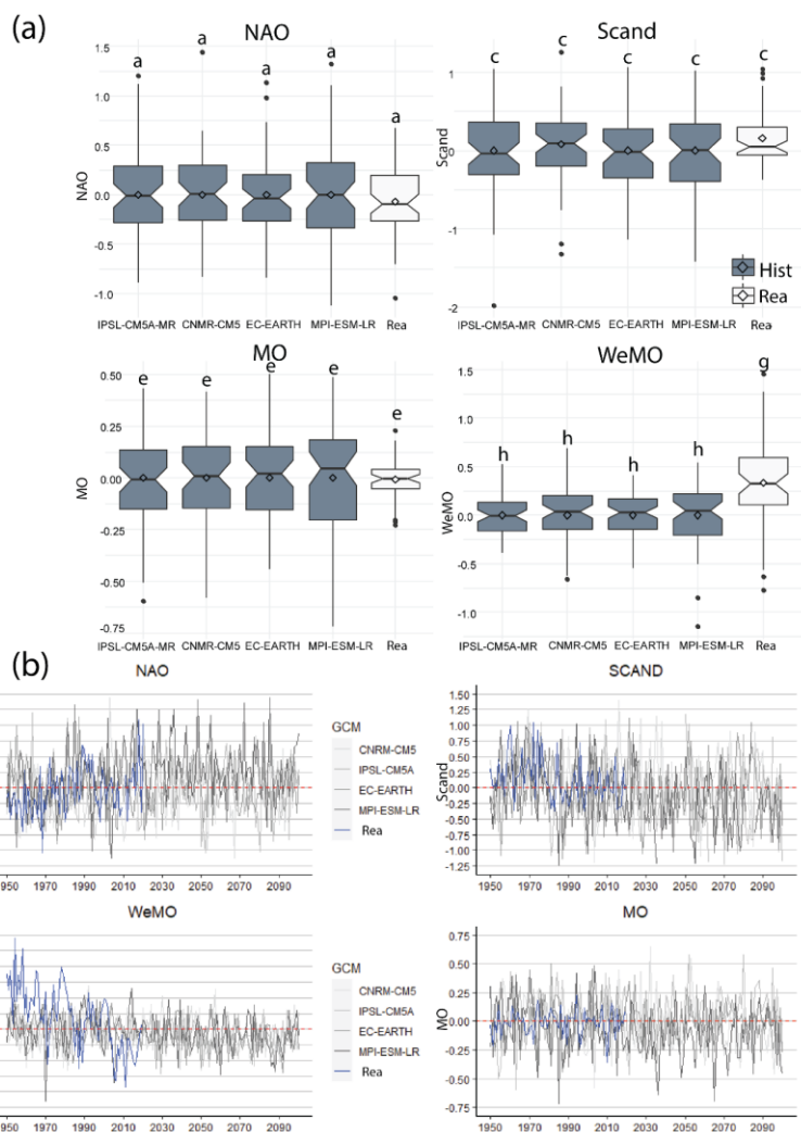
305 Figure 4: Evolution of the annual teleconnection pattern (a) Variability of teleconnection patterns provided by the reanalysis for the period 1950-2005 (Rea) and simulated by the 4 GCMs in the historical period 1950-2005 (Hist). Letters indicate whether box plots are significantly equal (same letter as box plot 'Rea') or not (b) Annual future projections under a scenario RCP 8.5. The blue line represents the annual reanalysis data and is referred as 'Rea' in the legend
