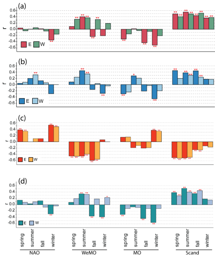
Figure 3: Estimated correlations between the teleconnection patterns and (a) RD103 (b) Water discharge (c) Temperature (d) Precipitation. For (a), (c), and (d) the period considered is 1959-2018, whereas in (b) the period considered is 1976-2018. Water discharge for each cluster is the sum of each river's water discharge for whose the watershed belongs to either one of the cluster. Thus, Western discharge is the sum of the Aude, Agly and Tet water discharge and eastern discharge the sum of Herault, Orb and Tech water discharge
