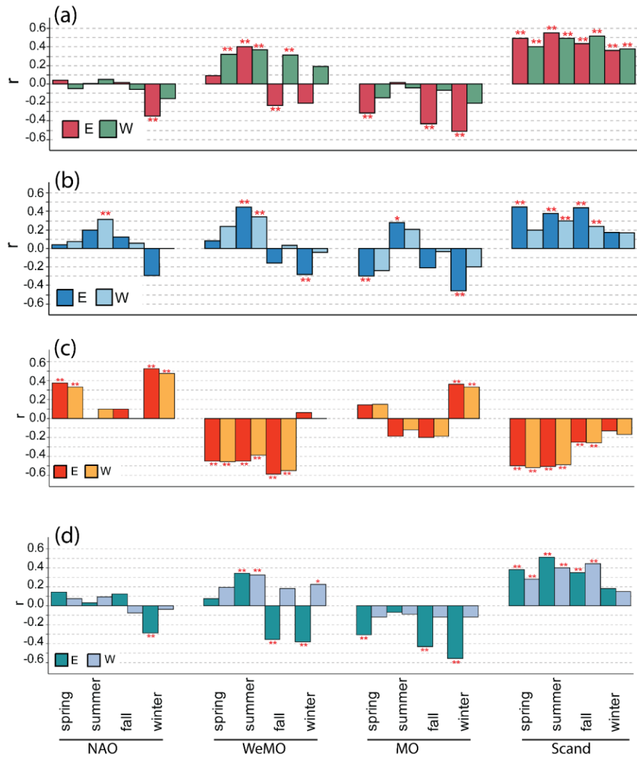
Figure 3: Estimated correlations between the teleconnection patterns and (a) RDI03 (b) Water discharge (c) Temperature (d) Precipitation. For (a), (c), and (d) the period considered is 1959-2018, whereas in (b) the period considered is 1976-2018. Water discharge for each cluster is the sum of each river's water discharge for whose the watershed belongs to either one of the cluster. Thus, Western discharge is the sum of the Aude, Agly and Tet water discharge and eastern discharge the sum of Herault, Orb and Tech water discharge
