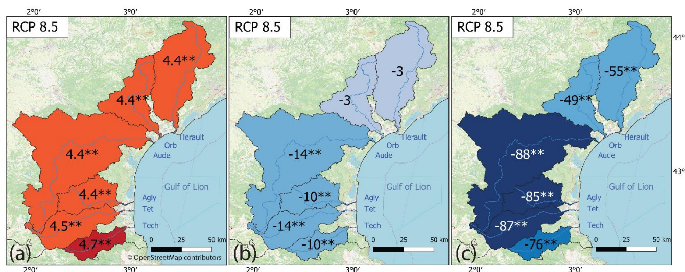
Figure 6: Linear trends for projected annual hydro-climatic variables under a scenario RCP 8.5 and for the period 2006-2100. Results are shown for the ensemble-mean of the 6 RCMs used in this study (a) temperature in °C (b) precipitation in % and (c) water discharge in %. Map data: © OpenStreetMap contributors 2021. Distributed under the Open Data Commons Open Database License (ODbL) v1.0.
