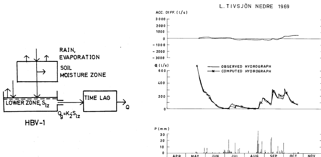
Figure 4. A sketch of the very first version of the HBV model and the very first successful simulation of runoff based on data from the Lilla Tivsjön basin (from Bergström, 1976).
