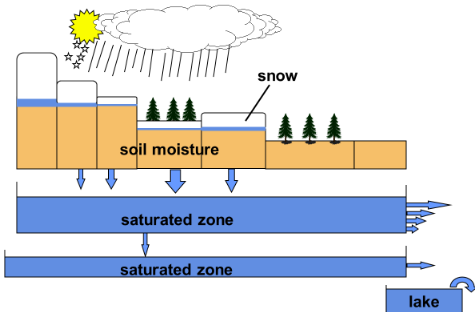
110 Figure 2. Structure of the HBV model (drawn by Sten Bergström).
