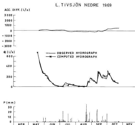
Figure 4. A sketch of the very first version of the HBV model and the very first successful simulation of runoff based on data from the Lilla Tivsjön basin (from Bergström, 1976).
