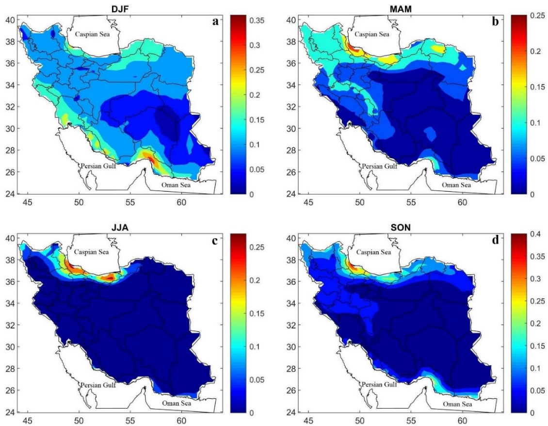
785 Figure 4. Cumulative dew yield [ \text{L/m}^2/\text{day} ] presented as an overall seasonal mean during 1979–2018. (a) winter (December, January, and February), (b) spring (March, April, and May), (c) summer (June, July, and August), and (d) autumn (September, October, and November).
