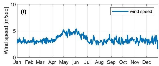
805 Figure 8. Night time (i.e. 18:00, 21:00, 00:00, 03:00) long term mean (1980-2010; 30 years) of wind speed in six selected stations that are located in dew zone A-F. (a) Ramsar (dew zone A); (b) Zanjan (dew zone B); (c) Isfahan (dew zone C); (d) Tabas (dew zone D); (e) Ahvaz (dew zone E), and (f) Bandarabas (dew zone F). Data were obtained from the meteorological organization of Iran.
