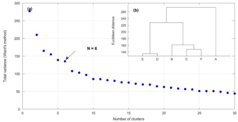
970 Figure 2. (a) Distance level at which two clusters are merged as function of the number of clusters result of the Ward linkage method applied to daily dew yield data from 1979-2018. N is the optimal number of clusters has been chosen for this study and (b) dendrogram of 6 clusters.
