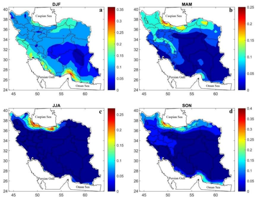
985 Figure 4. Cumulative dew yield [L/m 2 /day] presented as an overall seasonal mean during 1979–2018. (a) winter (December, January, and February), (b) spring (March, April, and May), (c) summer (June, July, and August), and (d) autumn (September, October, and November).
