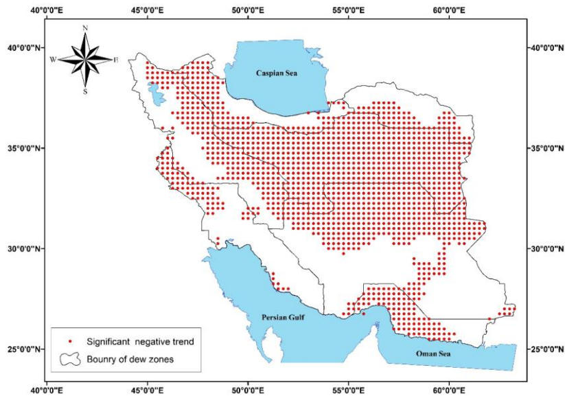
Figure 9. Mann-Kendal trend test on mean yearly dew yield over the years 1979- 2018 as predicted by Sen's slope estimator. Only locations with a statistically significant trend ( p < 0.05 ) are shown. Red points present locations with negative trend, regardless their decreased values and the white parts did not show any significant trend at ( p < 0.05 ).
