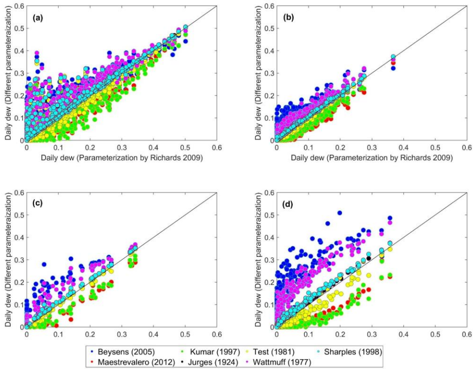
Figure 10. Scatter plots of daily dew yield obtained from parameterization by Richards (2009) against 7 different parameterizations listed in Table 6 for 4 stations in different areas of Iran. (a) Ramsar (forest and coastal area in the north); (b) Zanjan (mountains area); (c) Tabas (desert area in central Iran), and (d) Bandarabas (arid coastal area in the south). The black lines are the 1:1 relationship.
