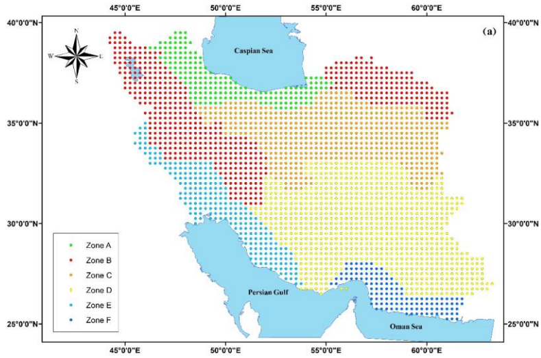
990 Figure 5. Dew formation zones based on the cluster analysis of the daily cumulative dew yield during 1979–2018.
