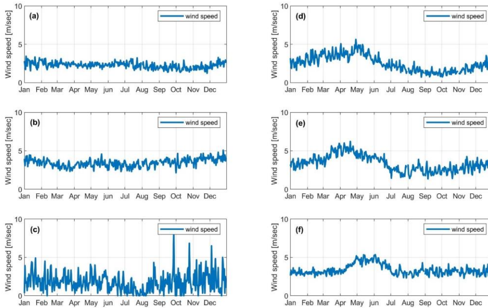
Figure 8. Night time (i.e. 18:00, 21:00, 00:00, 03:00), long term mean (1980-2010; 30 years) of wind speed in six selected stations that are located in dew zone A-F. (a) Ramsar (dew zone A); (b) Zanjan (dew zone B); (c) Isfahan (dew zone C); (d) Tabas (dew zone D); (e) Ahvaz (dew zone E), and (f) Bandarabas (dew zone F). Data were obtained from the meteorological organization of Iran.
