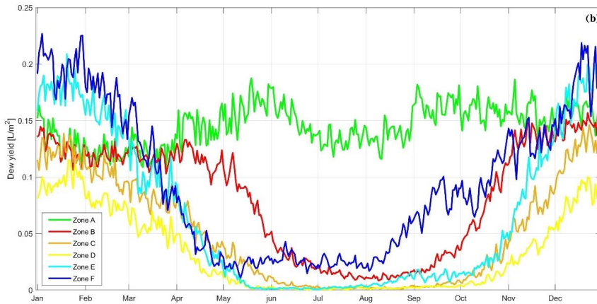
995 Figure 6. Long-term mean seasonal variation of the cumulative daily dew yield. Note that color coding on this figure is the same and corresponds to the dew formation zones on Figure 5: (Green) dew zone A (Caspian Sea), (red) Zone B (Zagros region), (orange) Zone C (Central Iran), (yellow) Zone D (Lut desert), (light blue) Persian Gulf zone, (dark blue) Oman Sea zone. The percentiles (i.e. 25%, median, 75% and 99%) of daily dew yields as average for each cluster are presented in Table 4.
