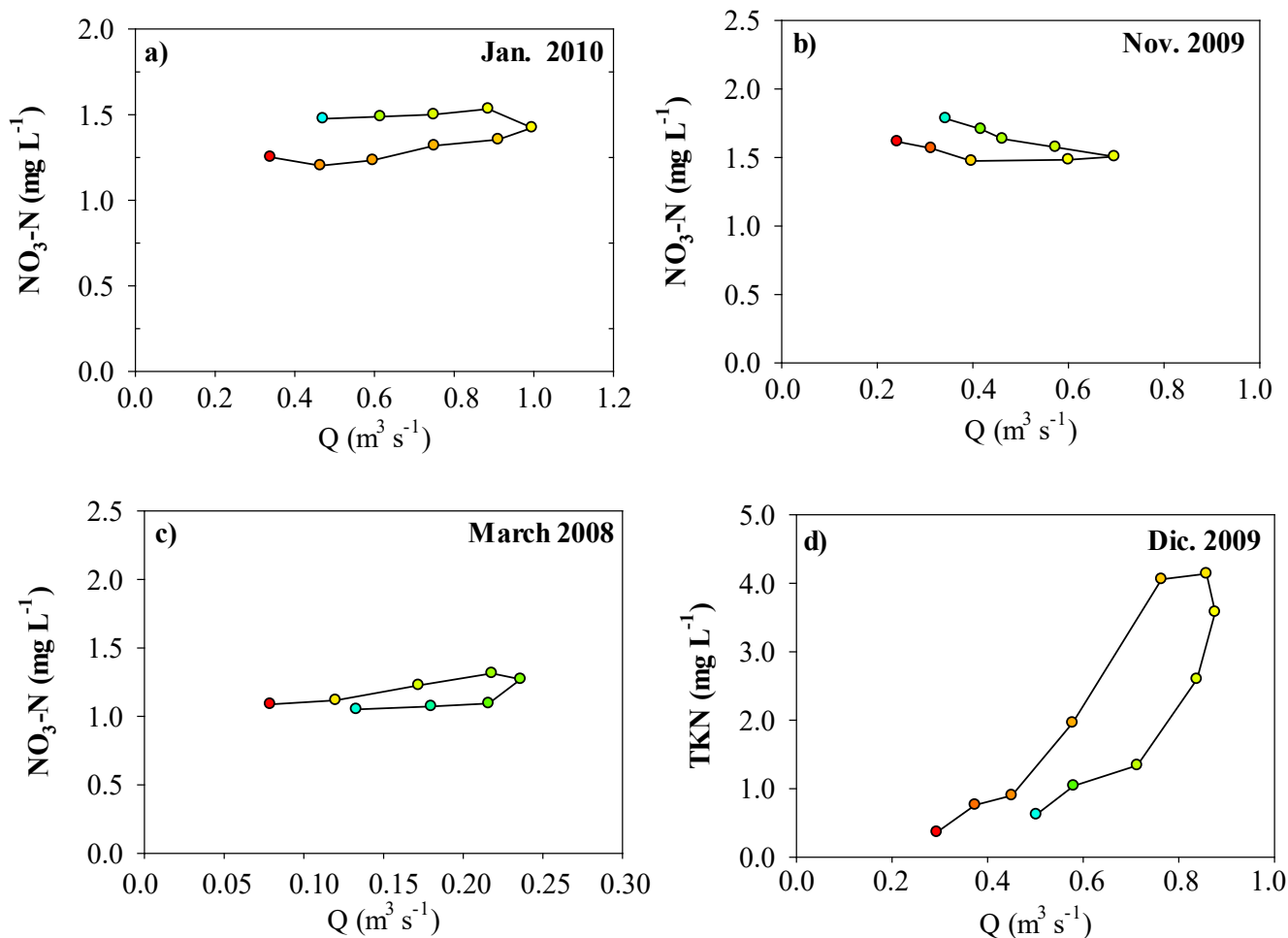
Figure 5: Examples of different types of \text{NO}_3^- (a, b and c) and TKN (d) hysteresis patterns observed in the Corbeira catchment during the monitoring period, where red indicates the start and blue the end of the runoff events. (a) Enrichment with anticlockwise pattern, (b) Dilution with anticlockwise pattern, (c and d) Enrichment with clockwise pattern. Circular arrows show the direction of clockwise and anticlockwise hysteresis.
