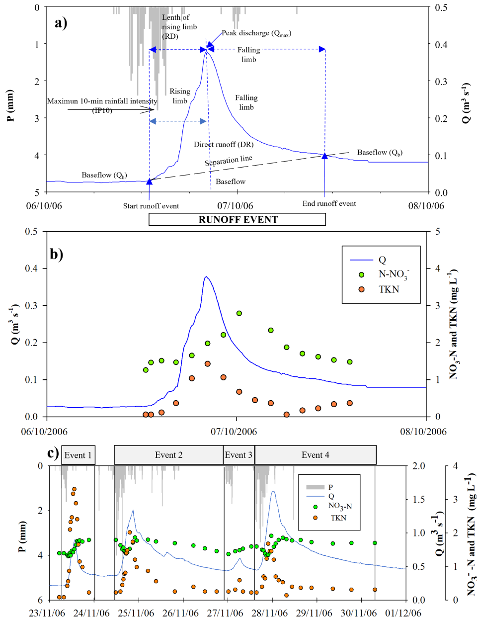
195 Figure 3: a) Diagram illustrating the hydrograph separation in two components (direct runoff and baseflow) using the constant slope hydrograph separation by Hewlett and Hibbert (1967). Some variable characteristics of the rainfall-runoff events are also indicated. b) Example of evolution of NO_3^- ( NO_3 -N) and TKN concentrations during a runoff event. c) Sequence of rainfall-runoff events and evolution of NO_3^- ( NO_3 -N) and TKN concentrations.
