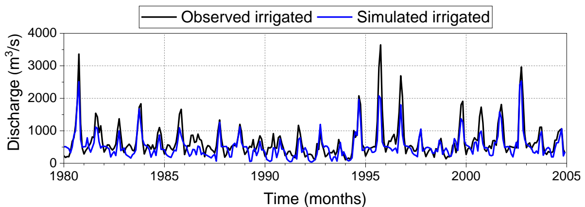
Figure S6: Monthly irrigated discharge hydrograph simulated by H08 model at Nakhon Sawan.
