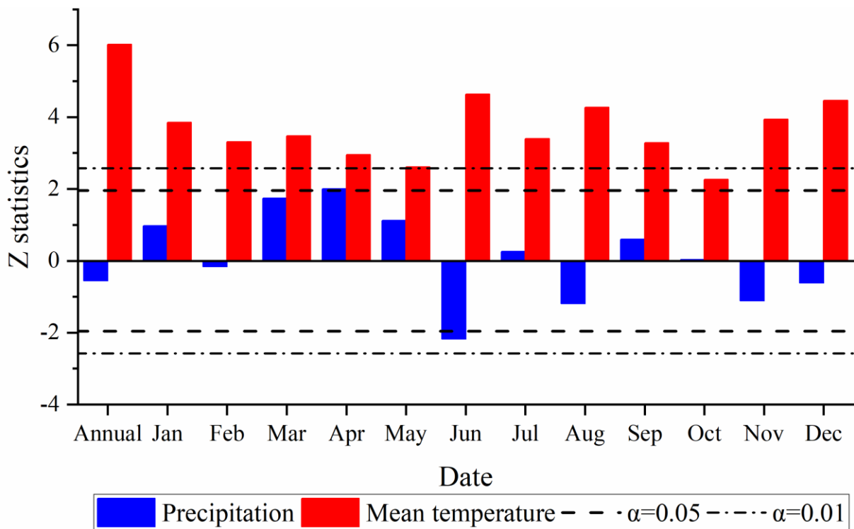
Fig. 7. The Mann-Kendall monotonic trend test statistics of the annual and monthly precipitation and mean temperature for the LR Basin from 1961 to 2015.
