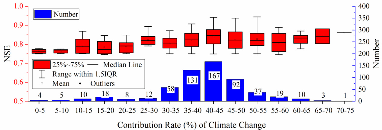
500 Fig. 10. Histogram of the number of simulations of the CR (with 5% steps) of climate change to streamflow reduction in the LR Basin at the annual scale and corresponding Nash-Sutcliffe Efficiency box plots.
