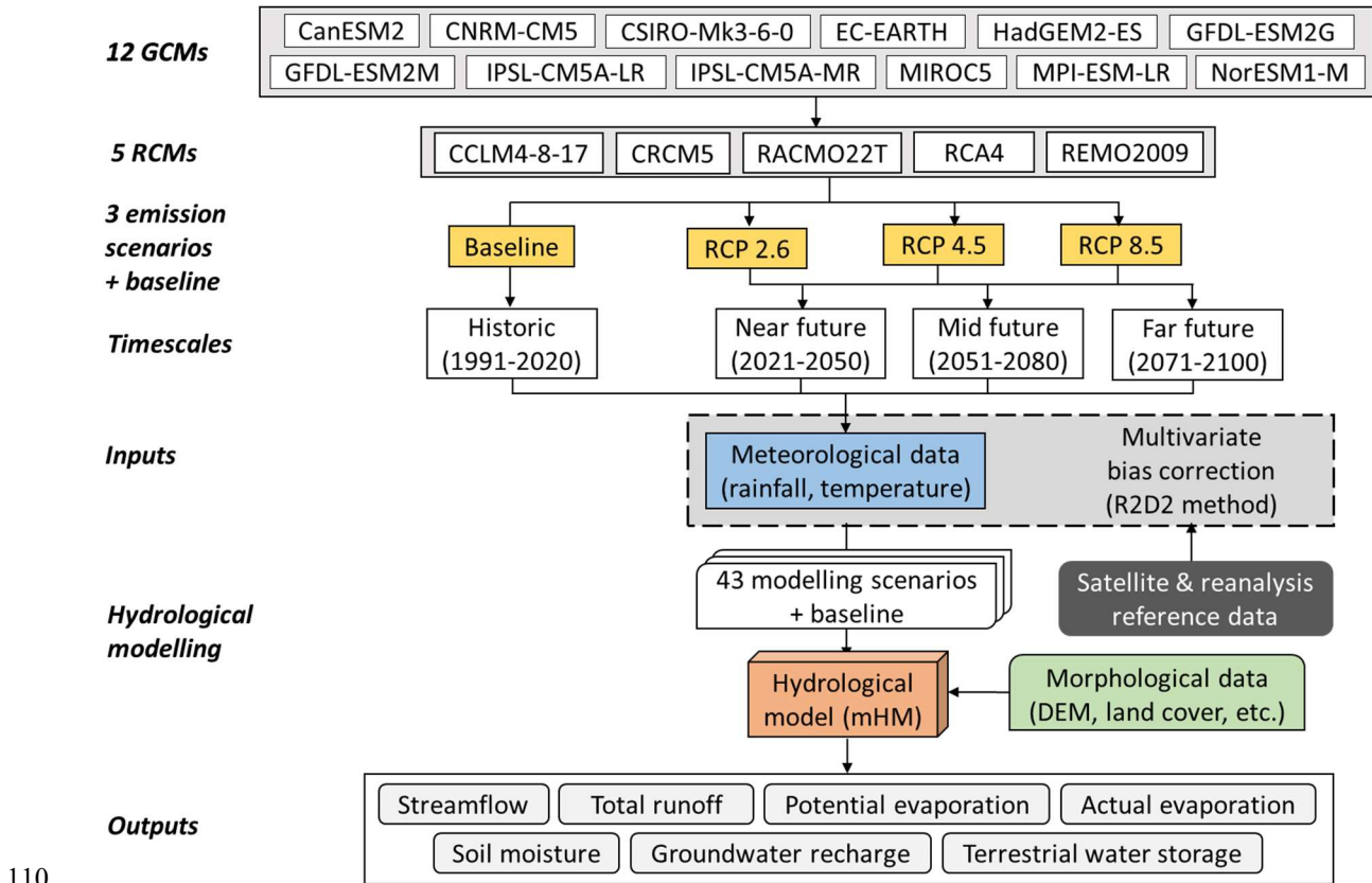
Figure 2. Overview of the procedure for assessing the impacts of climate change on hydrological processes.
