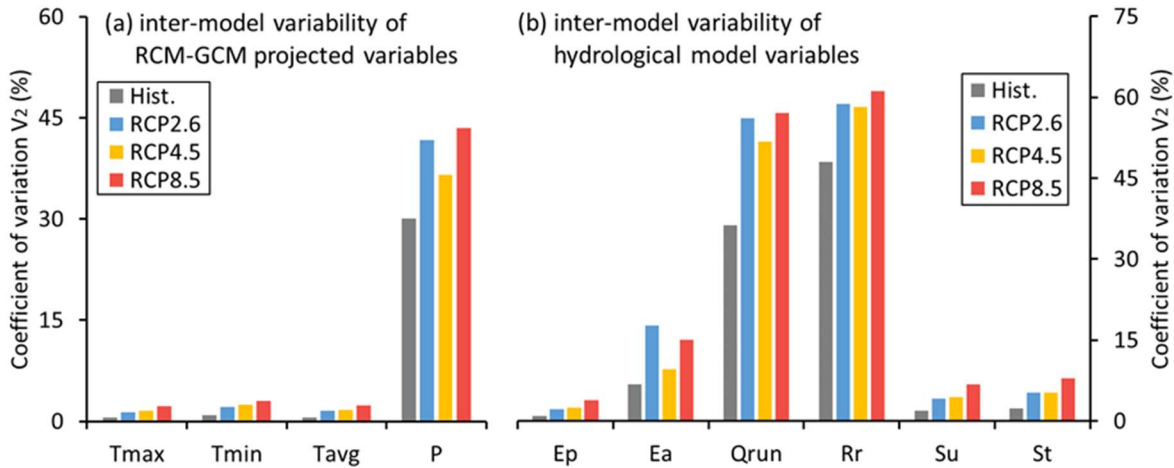
325 Figure 8. Average inter-model (i.e., RCM-GCMs) variability expressed with the second-order coefficient of variation ( V_2 ) for monthly hydroclimatic variables ( T_{max} , T_{min} , T_{avg} , P , E_p , E_a , Q_{run} , R_r , S_u , and S_t ) over the historical period (1991-2020) and the future period (2021-2100) under various RCPs.
