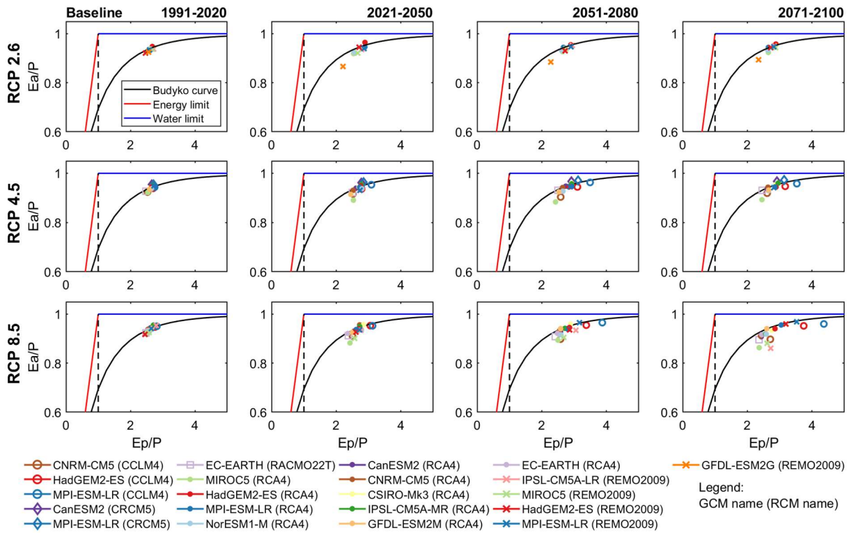
270 Figure 4. Plausibility of hydrological processes with the Budyko framework representing the evaporative index, i.e. ratio of actual evaporation to rainfall ( E_a/P ), as a function of the aridity index, i.e. ratio of potential evaporation to rainfall ( E_p/P ). The black dashed line represents the limit where precipitation equals potential evaporation.
