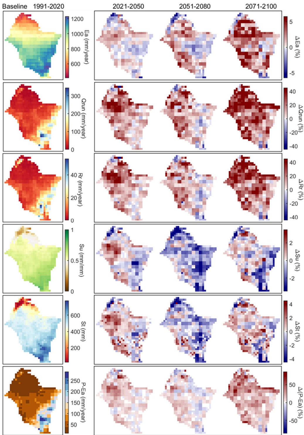
395 Figure 11. Spatial patterns of the long-term average of annual hydrological variables and water availability over the historical period (1991-2020) and changes over future periods (2021-2100) under RCP8.5 (median of 18 models).
