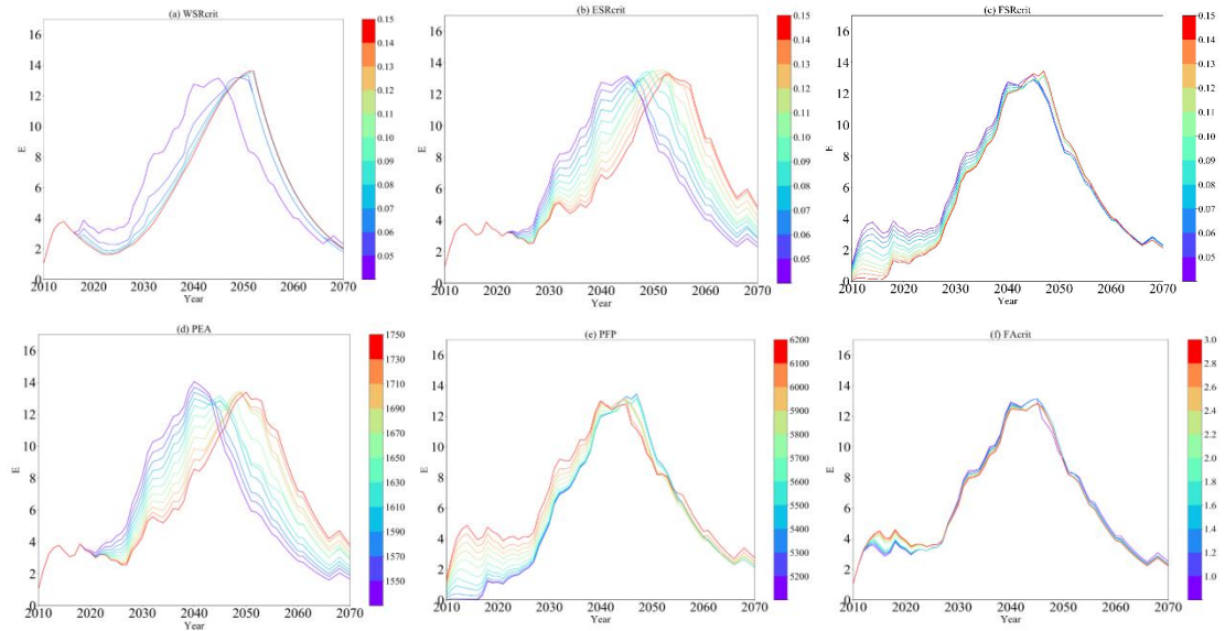
Figure 8. Trajectories of food production with varied parameters.
