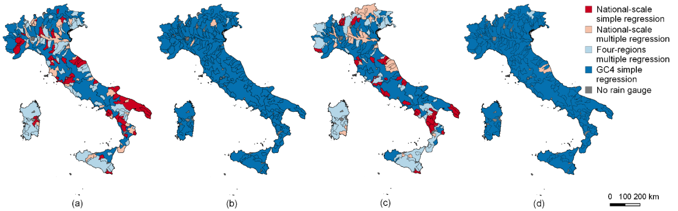
Figure 6. Absolute bias assessment for all the regression models used for the 1-hour case (a,b) and 24-hour case (c,d). The color refers to the model that provides the lowest absolute value of the bias. The GC4 model bias in cases (a) and (c) was only evaluated for statistically significant areas, while it was evaluated over every area in (b) and (d). Geomorphological data source: Alvioli et al. (2020).
