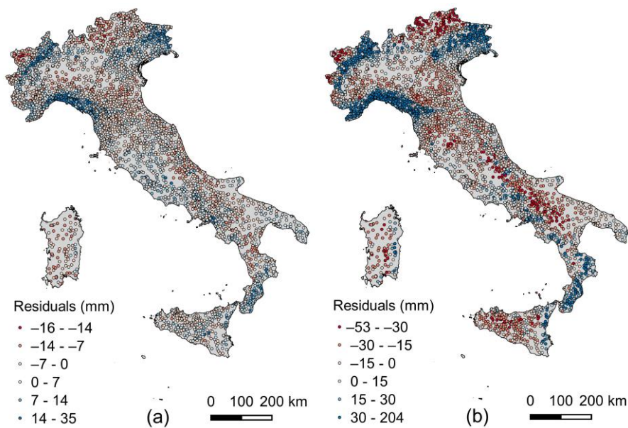
Figure 2. Residuals of the estimations of the 1-hour (a) and 24-hour (b) durations performed using Eqs. (3) and (5). Source: I 2 -RED data (Mazzoglio et al., 2020).
