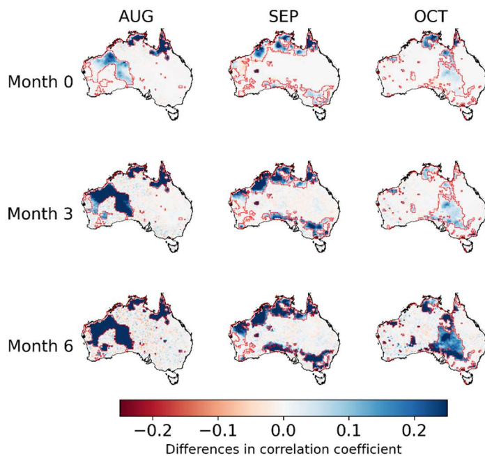
270 Figure 2. Differences in the correlation coefficient ( r ) between BJP-ti calibrated forecasts and observations with that between BJP calibrated forecasts and observations for three selected months (AUG, SEP, OCT) and three lead times (Months 0, 3, and 6). Red polygons show regions with significant observed trends.
