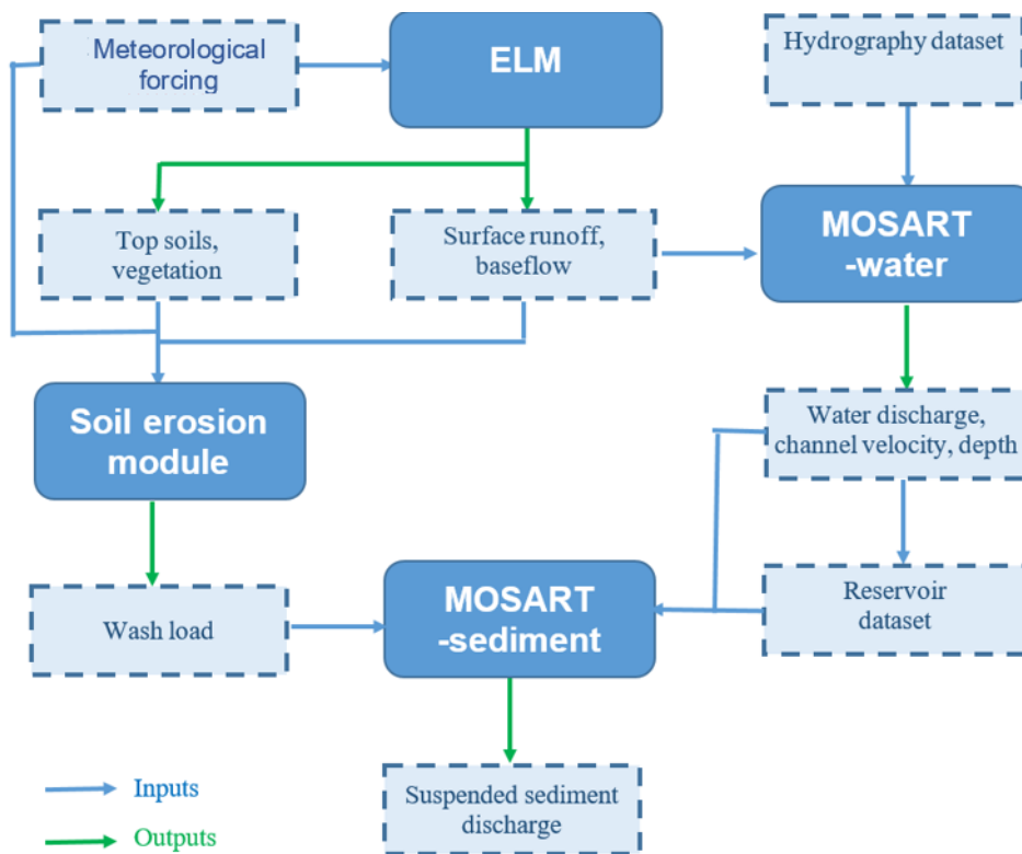
Figure 1: Modeling framework of MOSART-sediment.
