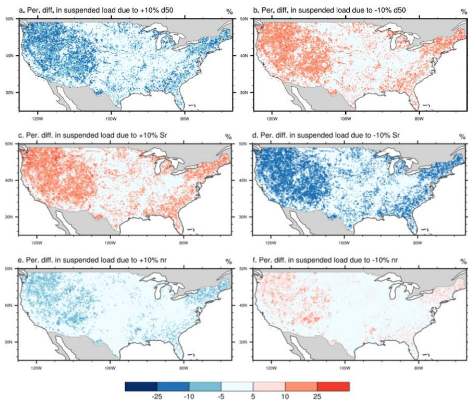
Figure 11: Spatial patterns of sensitivity of median bed-material size ( d50 ) (a, b), channel slope ( rs/p ) (c, d), and Manning's roughness for channels ( nr ) (e, f). At each grid, the percentage change of suspended load is calculated as 100\% \cdot (S_1 - S_0) / S_0 , where S_1 and S_0 are the average suspended load 1990-2012 simulated with the parameter changing by 10%, and the average suspended load simulated with the original parameters, respectively.
