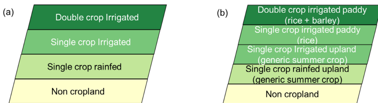
275 Figure 4 Grid cell categorization: a) the original categorization for global mode, and b) the new categorization for localized mode.
