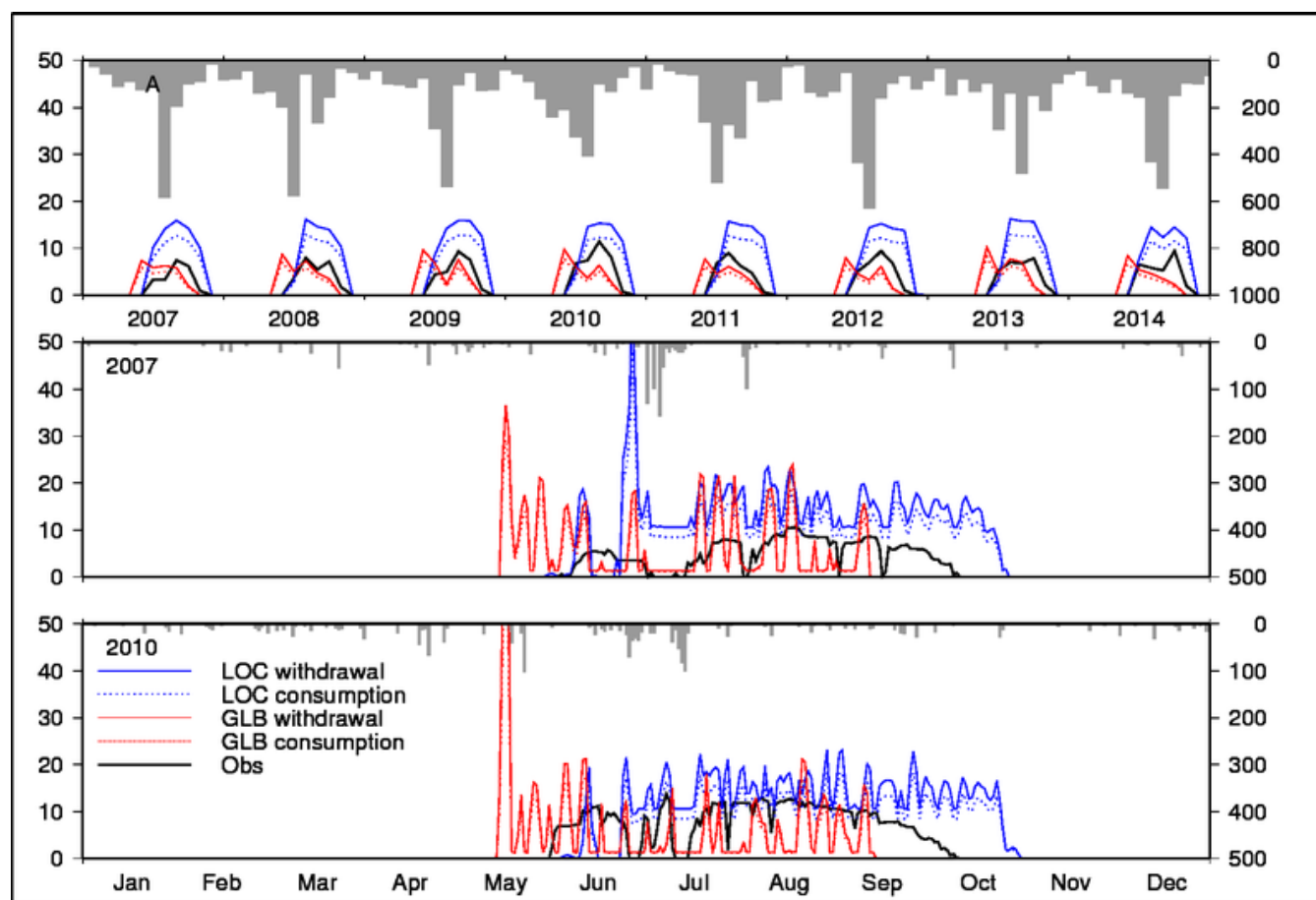
395 Figure 6 Irrigation water requirement at irrigation project A. Top: monthly time series of irrigation water withdrawal (lines) and basin-averaged precipitation from the LOC simulation (bars). Solid and broken lines indicate results including and excluding irrigation efficiency, respectively. Middle: daily time series of irrigation water and precipitation in the wettest year during the validation period. Bottom: daily time series of irrigation water and precipitation in the driest year during the validation period.
