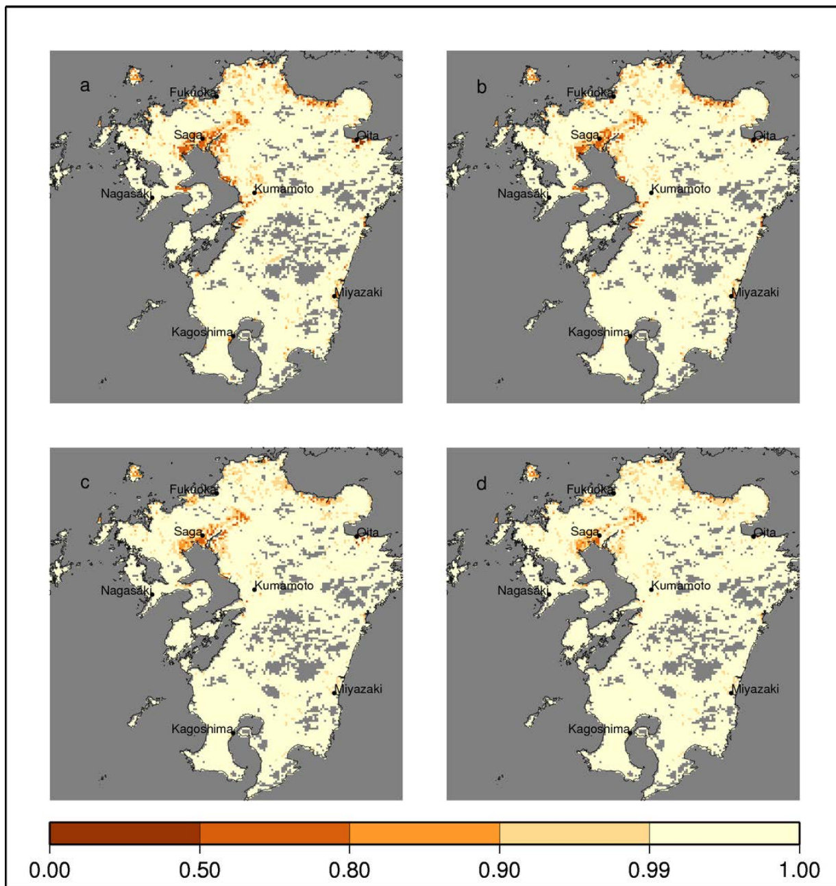
480 Figure 8 Water sustainability index. a) LOC-I1 (localized model with implicit aqueducts transferring water to 1 adjacent grid cell), b) LOC-I5 (localized model with implicit aqueducts transferring water to a maximum of five surrounding grid cells), c) LOC-I5O (localized model with implicit aqueducts transferring water to a maximum of five grid cells, including cells outside the basin), d) LOC-I5OE (localized model with implicit aqueducts transferring water to a maximum of five grid cells, including cells outside the basin as well as explicit aqueducts). Symbols show the centers of prefecture capital cities. For visibility, only mean annual withdrawal > 0.03 m 3 /s is shown.
