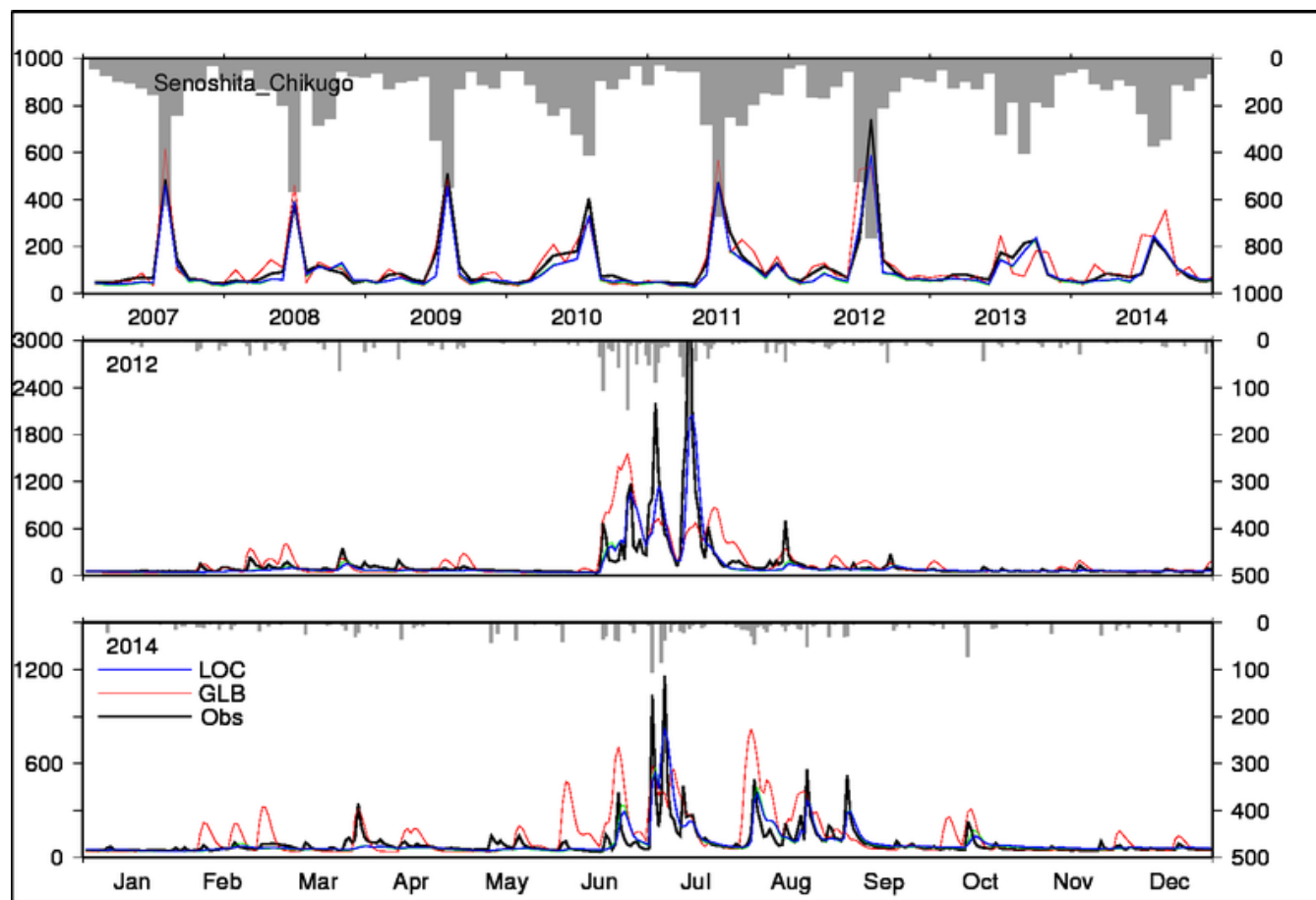
355 Figure 5 River discharge at Senoshita on the Chikugo River. Unit is \text{m}^3 \text{s}^{-1} . Top: monthly time series of streamflow (lines) and basin-averaged precipitation in the LOC simulation (bars). Middle: daily time series of streamflow and precipitation in the wettest year of the validation period. Bottom: daily time series of streamflow and precipitation in the driest year of the validation period.
