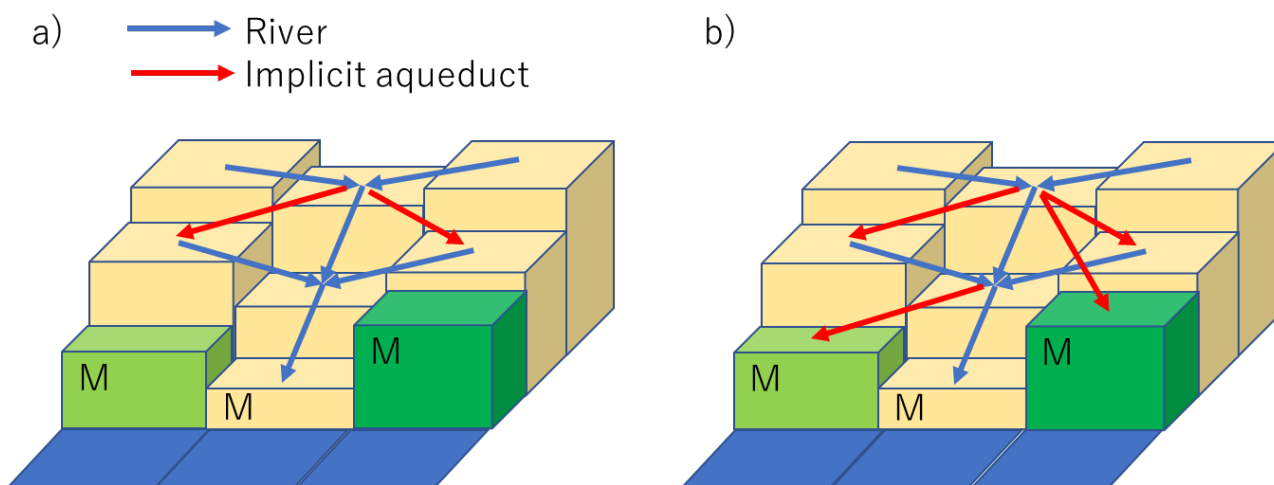
Figure 3 Implicit aqueducts. a) The original scheme, which does not allow inter-basin transfer. b) The new scheme, which conditionally allows inter-basin transfer. Columns represent land grid cells. The height indicates each grid cell's mean elevation. Colors indicate different basins. M denotes the grid cell containing the river mouth.
