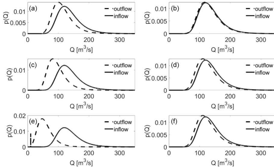
Figure 3. Derived probability density functions of the peak outflow obtained by modifying the height of the spillway crest ( h_s ) and the equivalent event duration t_p . Graphs on the left ( a , c , e ) are associated with a duration of half an hour and those on the right ( b , d , f ) to a duration of 1 h, while elevation of the crest changes between 2 ( a , b ), 4 ( c , d ) and 8 m ( e , f ). Other parameters are \alpha = 30 \text{ m}^3/\text{s} ; \beta = 120 \text{ m}^3/\text{s} ; b = 1 \text{ m} ; d = 1 \text{ m} ; n = 1.5 ; h_f = l_f + d/2 = 0.5 \text{ m} ; h_s = 2 ; \mu_f = 0.85 ; \mu_s = 0.385 ; L = 5 \text{ m} .
