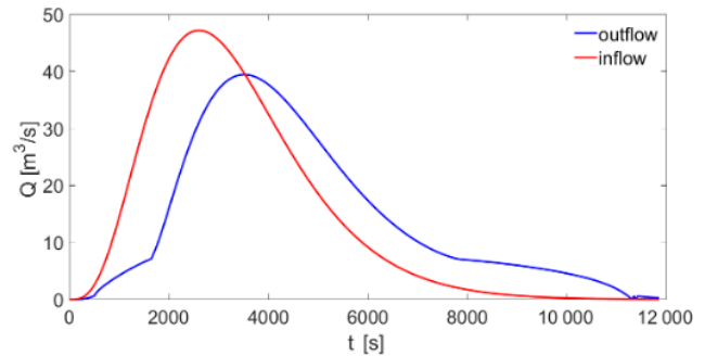
Figure 2. Example of flood mitigation induced by the presence of a detention basin obtained via numerical simulation. Other parameters are b = 1 m; d = 1 m; n = 1.9 ; h_f = l_f + d/2 ; h_s = 4 ; \mu_f = 0.85 ; \mu_s = 0.385 ; L = 3 m, W_{\max} = 15000 m 3 .
