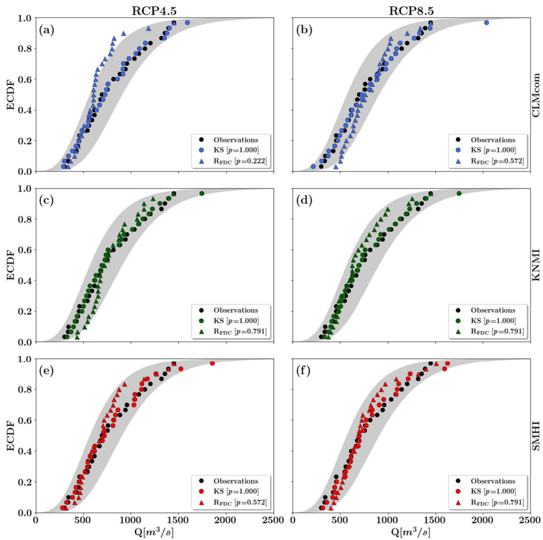
445 Figure 45: Simulated ECDFs of daily annual maximum streamflow at Trento the gauging station of Trento in the period 1982-2010 450 with precipitation and air temperature provided by CLMcom (first row), KNMI (second row), and SMHI (third row) climate models under the RCP4.5 (left) and RCP8.5 (right) emission scenarios. Calibration of HYPERstreamHS was performed using both KS and RFDC metrics as objective functions. The ECDF of observations is also shown with black dots together with the associated 90% confidence interval of the fitted Gumbel distribution (grey shaded area). p-values of the Kolmogorov-Smirnov two-sample test are also reported within brackets for each simulation run.
