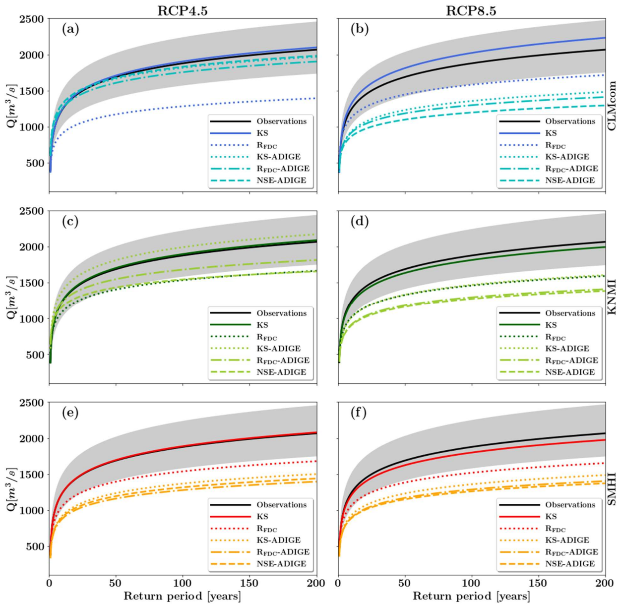
Figure 56: Quantiles of daily annual streamflow maxima as a function of return period at the Trento gauging station. Extrapolations are based on simulations conducted during the period 1982-2010 using as input forcing the CLMcom (first row), KNMI (second row), and SMHI (third row) climate models under the RCP4.5 (left) and RCP8.5 (right) emission scenarios, respectively. Each curve represents a combination of CM, emission scenario and parameterization obtained with the calibration. Simulations conducted using the parameterizations derived from obtained by using the use of observational dataset ADIGE as input in calibration are labelled as NSE-ADIGE, R FDC -ADIGE and KS-ADIGE. Extrapolation from observed streamflow maxima is also shown (continuous black line) together with the associated 90% confidence interval of the fitted Gumbel distribution (grey shaded area).
