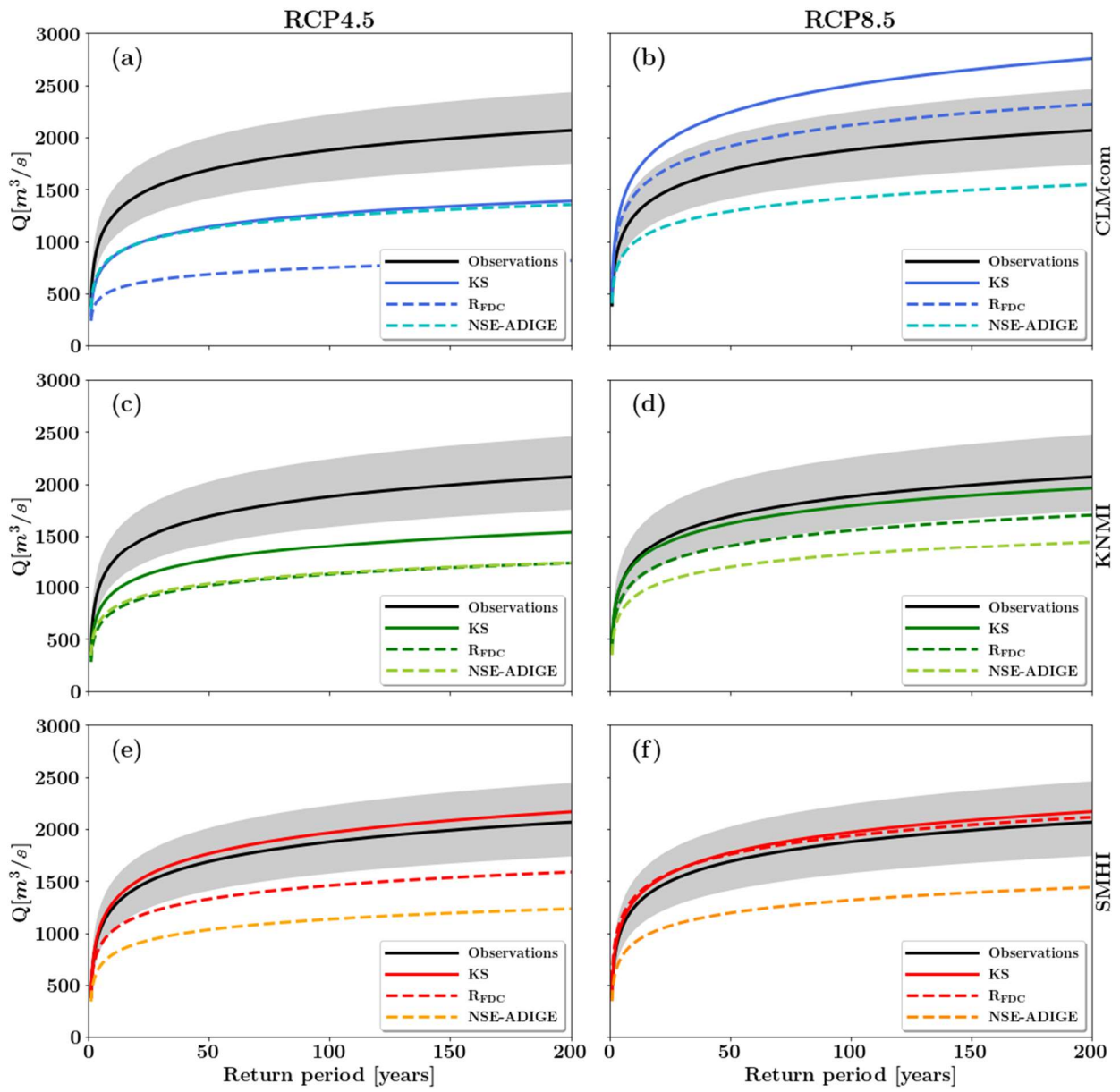
Figure 78: Quantiles of annual maximum daily streamflow as a function of return period at the Trento gauging station. Projections are based on simulations conducted during the future time period 2042-2070 using as input the CLMcom (first row), KNMI (second row), and SMHI (third row) climate models under the RCP4.5 (left) and RCP8.5 (right) emission scenarios, respectively. The continuous black line denotes the extrapolation quantile distribution of high flow extremes evaluated with the observational data in the period 1982-2010 together with the associated 90% confidence interval of the fitted Gumbel distribution (grey shaded area).
