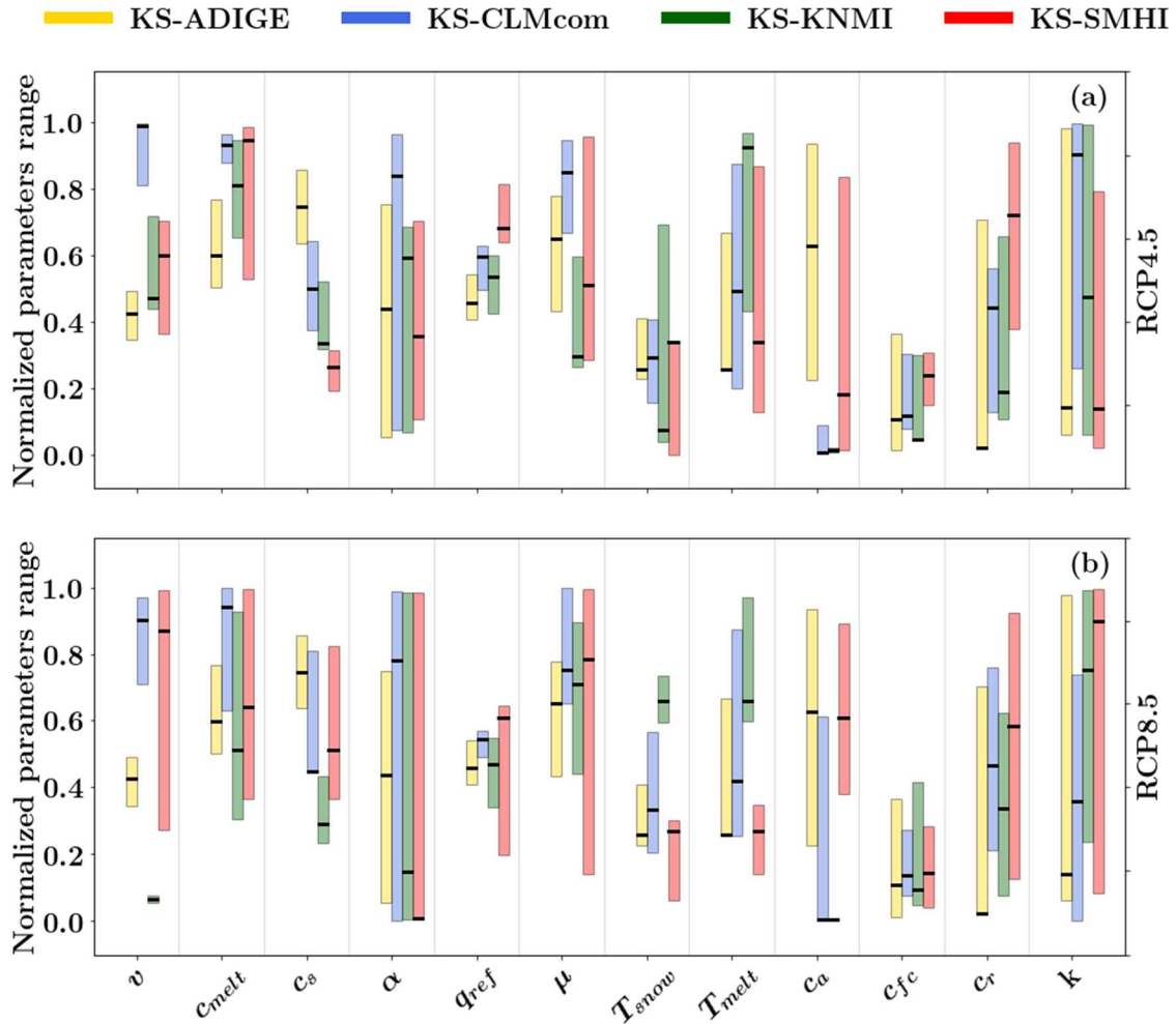
Figure 67: Range, \bar{d} , between the maximum and minimum value of each parameter associated with the 200 simulations presenting the highest efficiency plotted as a normalized range with respect to the parameter range presented in Table 1. Calibrations are conducted for the 3 different CMs under (a) RCP4.5 and (b) RCP8.5 emission scenarios with reference to the KS metric. Bold horizontal dashes indicate the optimal parameter sets for all experiments.
