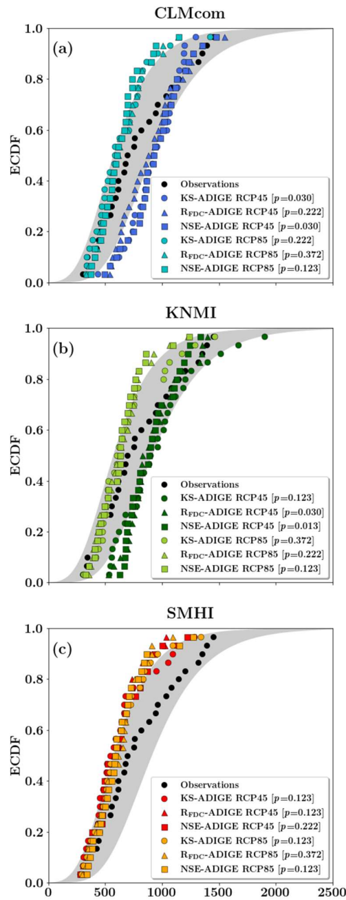
Figure 34: ECDFs of annual maximum streamflow at Trento gauging station in the period 1982-2010 obtained by using NSE-ADIGE, KS-ADIGE and R FDC -ADIGE parameterizations and a) CLMcom, b) KNMI, and c) SMHI climate models as input forcing for both RCP4.5 and RCP8.5 emission scenarios. The experimental ECDF-of-observations is also shown with black dots together with the associated 90% confidence interval of the fitted Gumbel distribution (grey shaded area). p-values of the Kolmogorov-Smirnov two-sample test are also reported within brackets for each simulation run.
