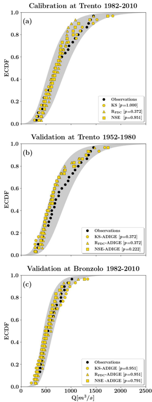
345 | Figure 23: ECDFs of daily annual streamflow maximum obtained by using as input the observational dataset ADIGE and the parametrizations NSE-ADIGE, KS-ADIGE and R FDC -ADIGE at a) the Trento gauging station in the period 1982-2010; b) the Trento gauging station in the period 1952-1980, and c) the Bronzolo gauging station during the period 1982-2010. The experimental ECDFs obtained from streamflow observations in the same time frames is are shown with black bullets with the grey shaded area indicating the associated 90% confidence interval of the fitted Gumbel distribution. p-values of the Kolmogorov-Smirnov two-sample test are also reported within brackets for each simulation run.
