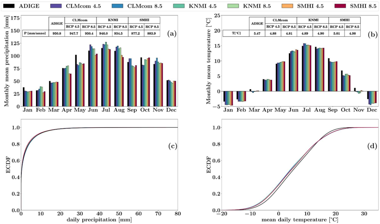
Figure 2: Annual cycle of basin-averaged monthly mean precipitation (a) and temperature (b) during the reference period 1980-2010 for both ADIGE and the 6 CMs used (different color bars). The associated annual averages are also shown in the insets. ECDFs of basin-averaged daily precipitation and temperature for the same datasets are presented in subplots (c) and (d), respectively.
