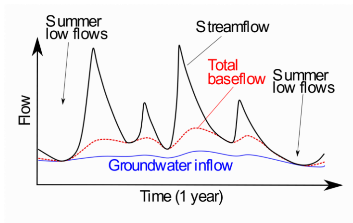
80 Fig. 1. Conceptualisation of baseflow. Over the water year, baseflow may dominate streamflows during successive low flow periods; however, groundwater inflows may be dominant only during low summer flows. Both the groundwater inflows and total baseflow are conceived to vary smoothly.
