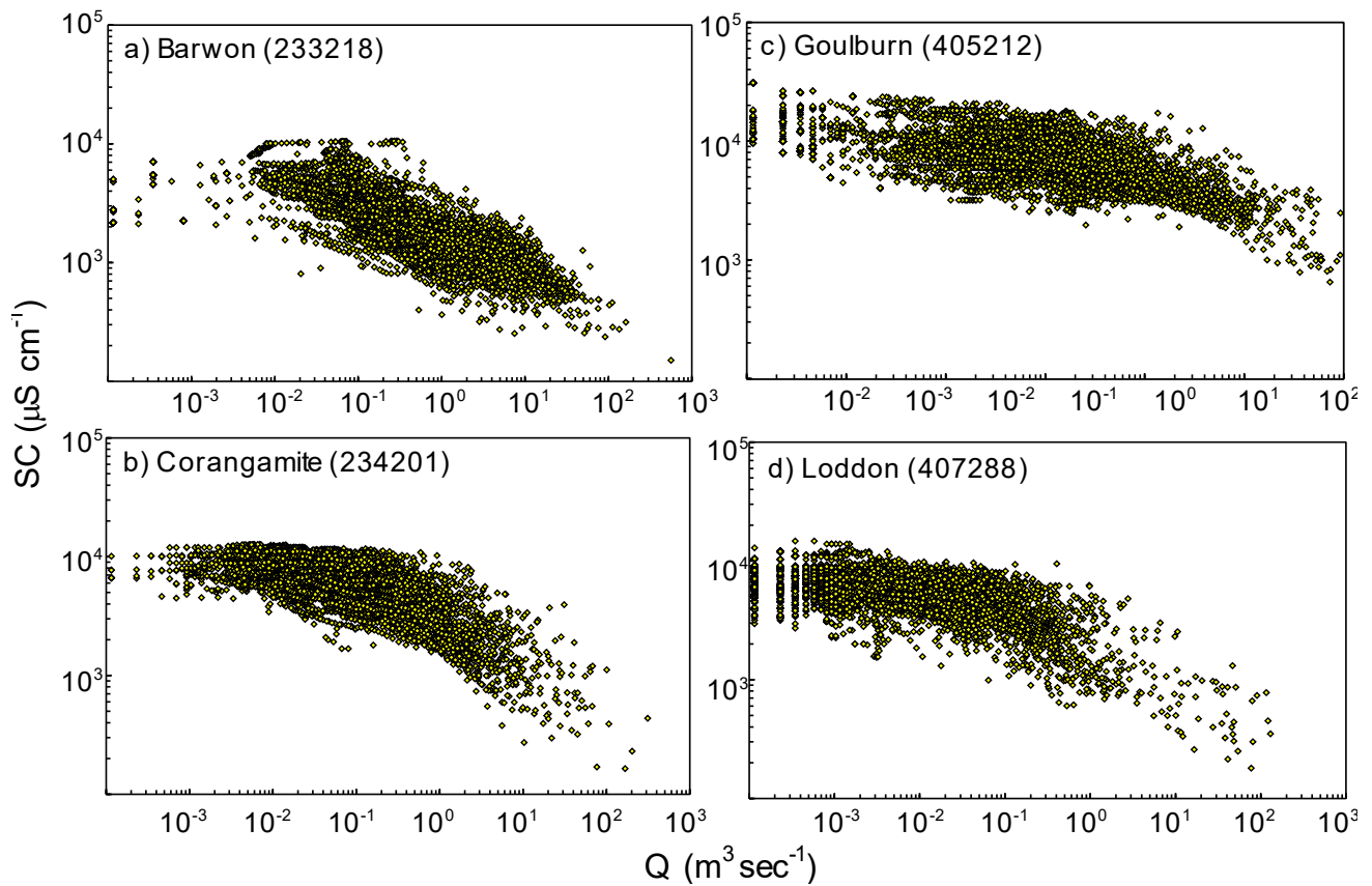
Fig. 3. Variation in streamflow (Q) and river SC for one station in the Barwon (3a), Corangamite (3b), Goulburn (3c), and Loddon (3d) catchments (data from Department of Environment, Land, Water and Planning, 2021).
