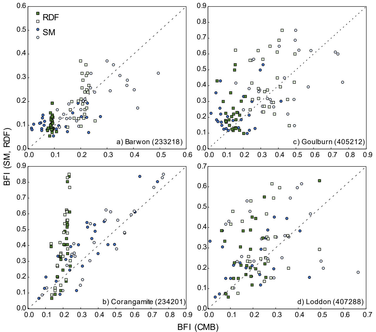
305 Fig. 5. Comparison of annual BFI estimates calculated from the RDF and SM methods with the BFI from the CMB using the variable (open symbols) and constant SC_b approach for one station in the Barwon (4a5a), Corangamite (5b), Goulburn (5c), and Loddon (5d) catchments. Dashed lines are the 1:1 relationship.
