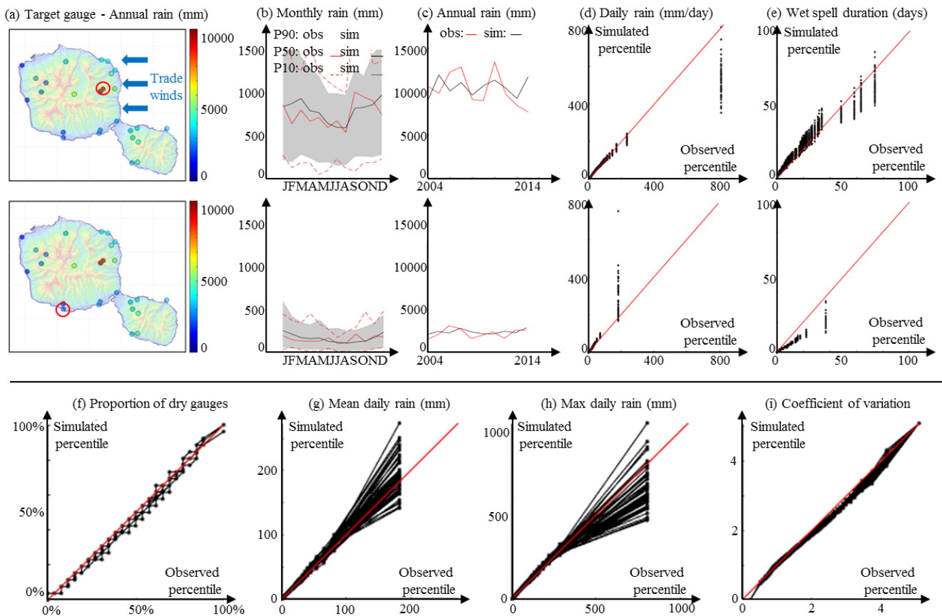
460 461 Figure 7: Overview of stochastic daily rainfall simulation for the island of Tahiti, French Polynesia. (a-e) Site-specific statistics: (a) 462 Target locations. (b) Observed (red) and simulated (black) monthly rain accumulation. (c) Observed (red) and simulated (black) annual rain 463 accumulation. (d) Q-q plot of daily rain percentiles. (e) Q-q plot of wet-spell duration percentiles. (f-i) Island-scale statistics: (f) proportion 464 of dry gauges; (g-h) mean and max daily rain; (i) coefficient of variation. 465
