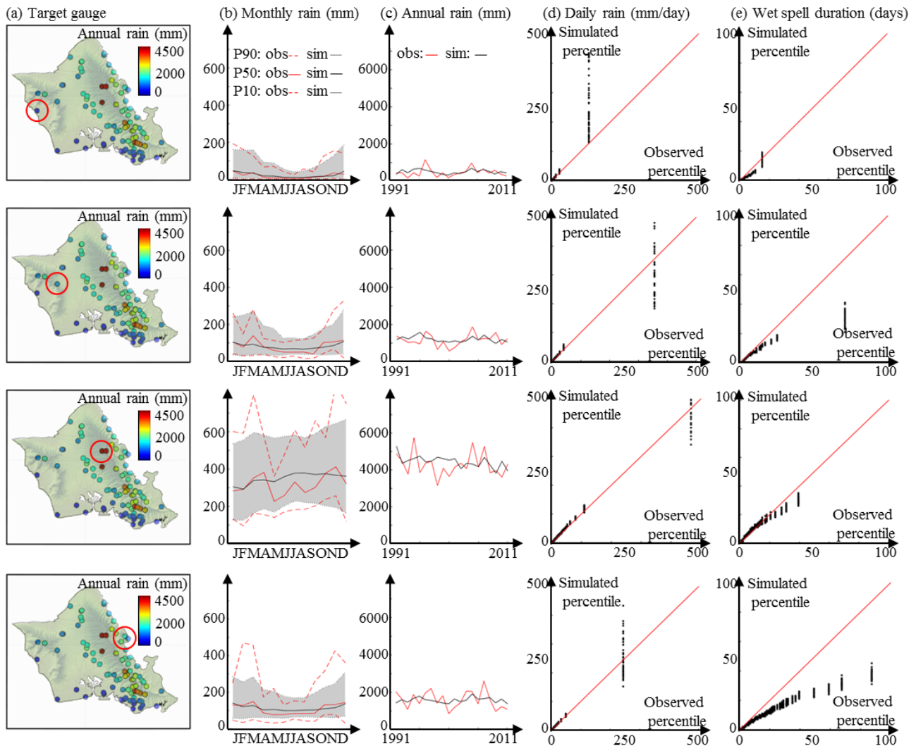
390 391 Figure 5: Ability of the model to simulate site-specific rain statistics on O'ahu. (a) Target locations. (b) Observed (red) and simulated 392 (black) monthly rain accumulation. Dashed lines denote quantiles 10% and 90%, and solid lines denote the quantile 50%. In the case of 393 simulations (black), for readability, we report in the figure only the median of each quantile (10%, 50%, 90%) instead of 50 simulated 394 quantiles. (c) Observed (red) and simulated (black) annual rain accumulation. In the case of simulations (black), for readability, we report in 395 the figure only the median of the 50 simulations. (d) Q-q plot of daily rain percentiles. (e) Q-q plot of wet-spell duration percentiles. Black 396 dots line up vertically in q-q plots (d–e) because for each percentile, 50 simulations are compared to a single observation.
