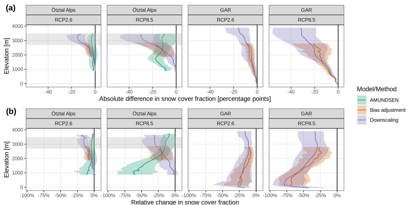
515 Figure 6. Change in future snow cover fraction (SNC) for the Ötztal Alps region and the whole study area (GAR, Greater Alpine Region) by elevation band. Colored lines and transparent regions denote model means and model spread from running a snow and hydroclimatological model (AMUNDSEN), forced by downscaled meteorology from regional climate models (RCMs), from bias adjusted SNC from RCMs, and from downscaled SNC from RCMs. Shaded grey area in the Ötztal Alps panels (above 2700 m) indicates elevations, where >20 % of the pixels entering the average per elevation band were removed from MODIS and Downscaling but remained included in AMUNDSEN: these consist of glacierized pixels or pixels subject to snow accumulation in RCMs, while AMUNDSEN resolved the whole domain. (a) shows absolute changes and (b) relative changes.
