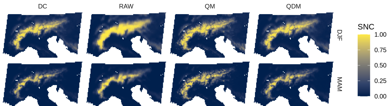
360 Figure 4. Average seasonal snow cover fraction (SNC), as observed from remote sensing (OBS) and simulated with the CLMcom-CCLM4-8-17 regional climate model driven by CNRM-CERFACS-CNRM-CM5 under the RCP8.5 emission scenario. Abbreviations: remotely sensed observations (OBS), raw climate model output (RAW), quantile mapping (QM), quantile delta mapping (QDM), delta change approach (DC), December-January-February (DJF), March-April-May (MAM). For maps of the other climate models and emission scenarios, see (Matiu, 2021).
