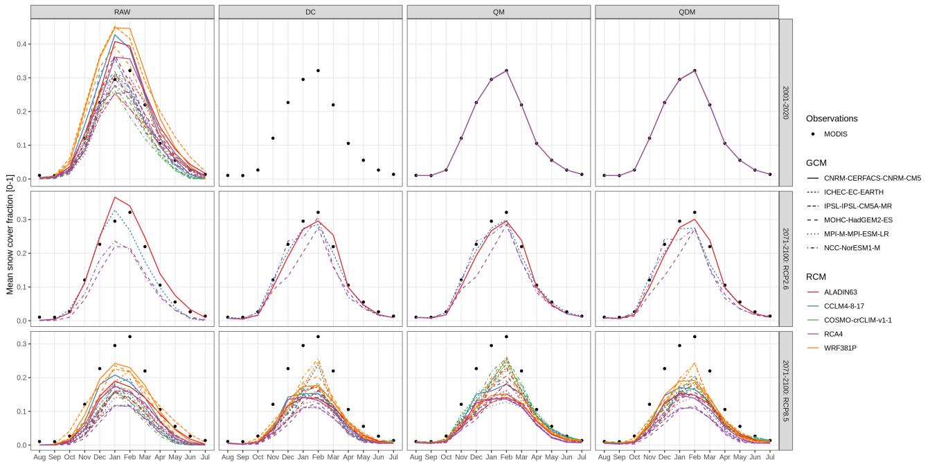
355 Figure 3. Average monthly snow cover fraction over the whole study domain before and after bias adjustment. Black points denote observations from remote sensing for the period 2001-2020 (the same in all panels), and colored lines the regional climate model (RCM) simulations with associated general circulation model (GCM). First row shows monthly averages for the past (2001-2020), while the middle and last row are for 2071-2100 averages for two emission scenarios (RCP, representative concentration pathway). Column RAW is for original RCM output, DC is the delta change approach, QM is quantile mapping, and QDM quantile delta mapping. Panel for DC and 2001-2020 shows no lines, since DC has no past RCM observations of its own.
