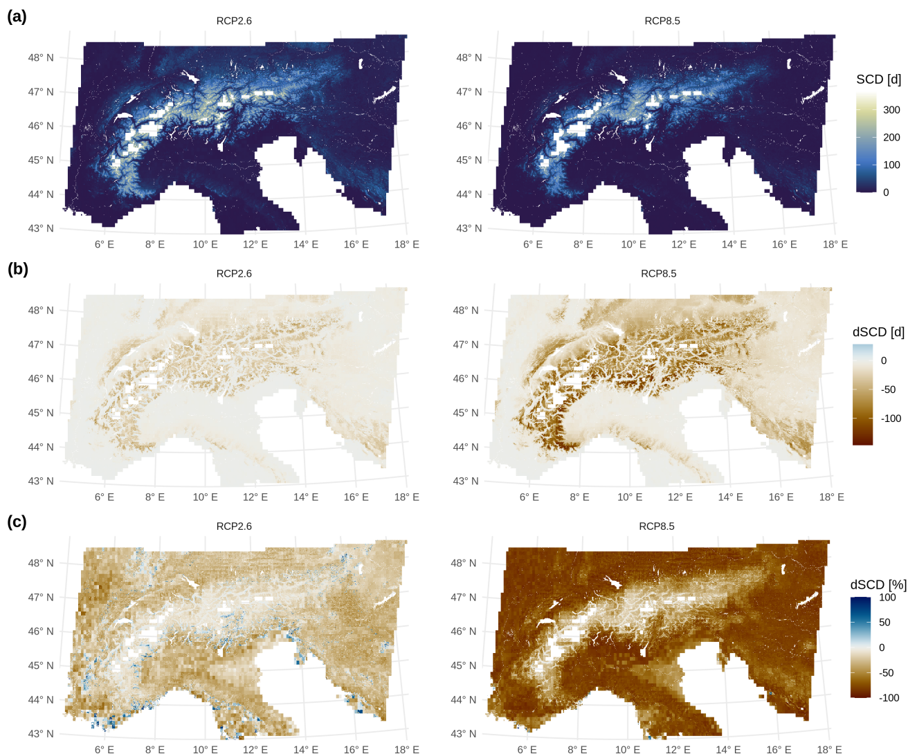
420 Figure 5. Future 2071-2100 annual snow cover duration (SCD) maps and differences to past (dSCD). (a) Downscaled SCD maps for low and high emission scenarios (RCP, representative concentration pathway) based on an ensemble of 4 models for RCP2.6 (regional climate models driven by general circulation models) and 23 models for RCP8.5. Empty areas denote pixels removed because of snow accumulation issues (see methods), glaciers, or water bodies. (b) Differences between future (2071-2100) and past (2001-2020) model output in absolute days. (c) Relative differences; pixels with > +100% difference omitted, because low values of 425 observed SCD caused noise in relative estimates for low SCD (most of the remaining positive changes are for areas with SCD ≤ 5 d, too).
