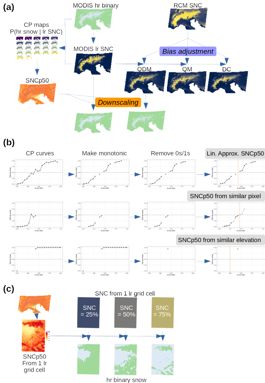
210 Figure 2. (a) Overview of methodology. (b) Detailed view of the estimation of SNCp50 based on CP curves. CP curves show the probability of the respective pixel being snow covered as a function of the encompassing grid cell SNC. (c) Downscaling exemplified at one low-resolution (lr) grid cell. The SNCp50 values determine the conversion from lr SNC to hr binary snow, which is shown for three example SNC values. Abbreviations: lr (low-resolution), hr (high-resolution), SNC (snow cover fraction), RCM (regional climate model).
