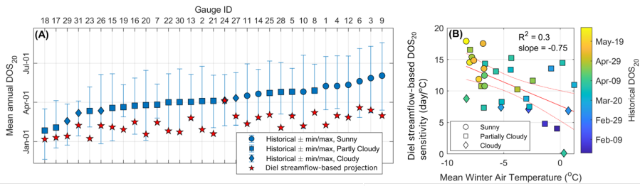
975 Figure 8: (A) Historical DOS_{20} from the diel analysis and projected changes in DOS_{20} using the empirical diel streamflow-based projections under the RCP 8.5 pseudo global warming climate for the end of the 21 st century. Watersheds are sorted from earlier (left) to later (right) historical DOS_{20} . Symbols associated with future projections (stars) are not classified by sunny, partly cloudy, or cloudy, as we make no inference about the cloudiness condition of snowmelt days under the climate change scenario. Blue symbols in (A) represent the mean annual percentage of clear-sky snowmelt days, where sunny sites (circles) have >90% clear-sky snowmelt days, partly cloudy sites (squares) have between 70 and 90%, and cloudy sites (diamonds) have <70%. Clear-sky snowmelt days are defined as those with more than 80% of the potential clear-sky solar radiation. (B) Relationship between mean winter air temperature and the sensitivity of DOS_{20} to climate change as projected by the empirical diel streamflow-based model. 980
