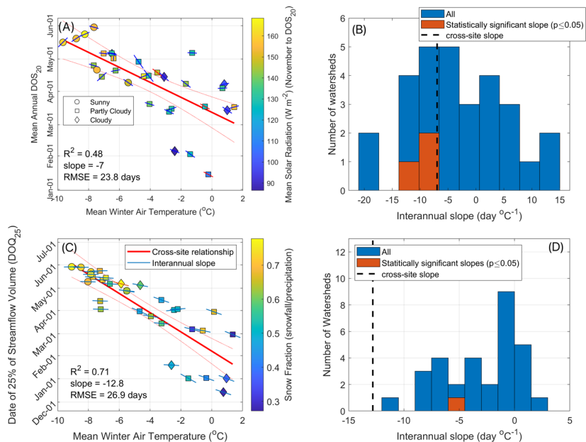
920 Figure 3: (A) and (C) show cross-site relationships between mean winter air temperature (November to February) and DOS 20 and the date of 25% of annual streamflow volume (DOQ 25 ), respectively. Slopes of individual sites' interannual relationships are shown as the lines on top of each symbol, where statistically significant ( p -value \leq 0.05 ) slopes are red. Non-significant interannual slopes are presented to show the overall tendency in their spatial distribution. Symbols are associated with the mean annual percentage of snowmelt days under clear-sky conditions. Sunny sites (circles) have >90\% clear-sky snowmelt days, partly cloudy sites (squares) have between 70 and 90%, and cloudy sites (diamonds) have <70\% clear-sky snowmelt days. Clear-sky snowmelt days are defined as those with more than 80% of the potential clear-sky solar radiation. (B) and (D) show histograms of interannual slopes (for all watershed and those with statistically significant relationships) and the cross-site relationships presented in their respective left panel. 925
