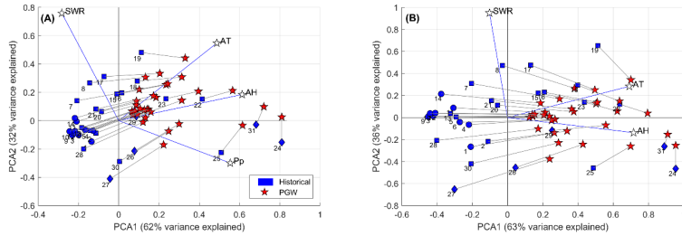
1055 Figure A6: (A) Principal Component Analysis for historical precipitation (Pp), air temperature (AT), absolute humidity (AH) and shortwave radiation (SWR) at each watershed, and the changes associated with the pseudo global warming as simulated by WRF. (B) shows the same analysis but excluding precipitation from the analysis. Blue symbols (circle, square and diamond) associated with historical values represent the mean annual percentage of clear-sky snowmelt days, where sunny sites have >90% clear-sky snowmelt days, partly cloudy have between 70 and 90%, and cloudy have <70%; clear-sky snowmelt days are defined as those with more than 80% of the potential clear-sky solar radiation. We make no inference about the cloudiness condition during snowmelt days under the RCP8.5 pseudo global warming scenario, and thus, we use a five-point star (in red) for the future scenario. Numbers next to blue symbols represent the Gauge IDs as presented in Table 2. 1060
