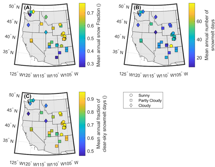
1030 Figure A3: (A): CAMELS mean annual snow fraction (snowfall/precipitation), (B) mean annual number of snowmelt days between 1031 December 1 and August 1 (calculated as the days with a correlation between hourly solar radiation and lagged streamflow greater 1032 than 0.8), and (C) mean annual fraction of clear-sky snowmelt days, calculated as the number of snowmelt days with clear-sky 1033 conditions as a fraction of total snowmelt days. A clear-sky snowmelt day is defined as having more than 80% of the potential clear- 1034 sky solar radiation. Symbols (circle, square and diamond) represent the mean annual percentage of clear-sky snowmelt days, where 1035 sunny sites have >90% clear-sky snowmelt days, partly cloudy have between 70 and 90%, and cloudy have <70.
