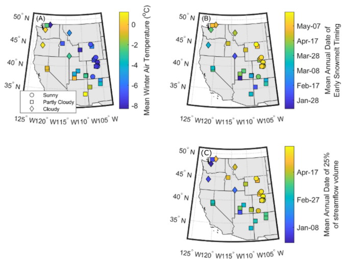
1025 Figure A2: (A): CAMELS mean winter (November to February) air temperature, (B) mean annual DO_{S_{20}} , and (C) mean annual DO_{Q_{25}} . Symbols (circle, square and diamond) represent the mean annual percentage of clear-sky snowmelt days, where sunny sites have >90% clear-sky snowmelt days, partly cloudy have between 70 and 90%, and cloudy have <70%; clear-sky snowmelt days are defined as those with more than 80% of the potential clear-sky solar radiation.
