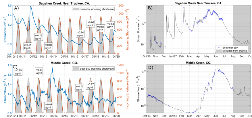
905 Figure 1: Examples of the diel cycle analysis applied to two watersheds located in California (A) (B) (WY2016) and Colorado (C) (D) (WY2014). (A) and (C) show hourly solar radiation (orange) and streamflow (blue); the first statistically significant ( p < 0.01 ) lagged spearman correlation ( r > 0.6 ) between streamflow and solar radiation is shown on a text box for clear-sky days only (>80% of clear-sky solar radiation). (B) and (D) show the solar radiation-driven snowmelt days (blue circles) on top of the annual hydrograph (semi-log scale) for the period of analysis (white background, December to July).
