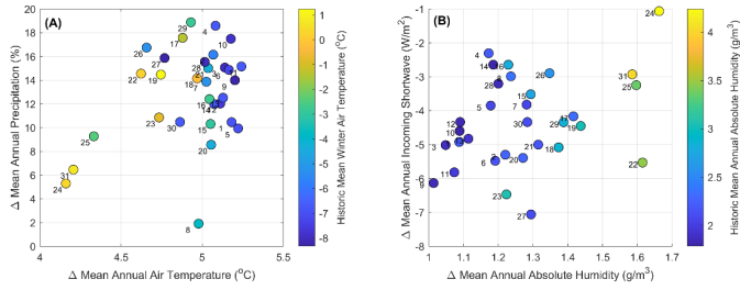
1050 Figure A5: Mean annual climate changes projected by WRF under an RCP8.5 pseudo global warming scenario by the end of the century. (A) shows changes in precipitation against air temperature. (B) shows incoming shortwave against absolute humidity. Numbers represent the Gauge IDs as presented in Table 2.
