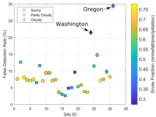
910 Figure 2: Percentage of days that were classified as having snowmelt following the diel streamflow cycle analysis that also had daily precipitation above 5 mm and a mean daily air temperature above 2 °C. Symbols are associated with the mean annual percentage of snowmelt days under clear-sky conditions. Sunny sites (circles) have >90%, clear-sky snowmelt days, partly cloudy sites (squares) have between 70 and 90%, and cloudy sites (diamonds) have <70% clear-sky snowmelt days. Clear-sky snowmelt 915 days are defined as those with more than 80% of the potential clear-sky solar radiation.
