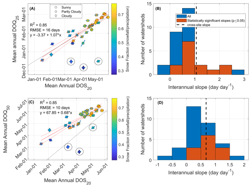
945 Figure 5: (A) The day when the 20 th percentile of snowmelt days occurs ( \text{DOS}_{20} ), compared to the date of the 25% of the annual streamflow volume ( \text{DOQ}_{25} ). (C) \text{DOS}_{20} against the date of 50% of the annual streamflow volume ( \text{DOQ}_{50} ). Dashed lines in (A) and (C) are 1:1 lines, and the slopes of sites' interannual relationships are shown as the lines on top of each symbol, with statistically significant ( p\text{-value} \leq 0.05 ) slopes shown in red. Sites #24, #25 and #31, indicated by dashed circles, fall far from the linear regression and are not included in its calculation. Symbols indicate the mean annual percentage of clear-sky snowmelt days, where sunny sites (circles) have >90% clear-sky snowmelt days, partly cloudy sites (squares) have between 70 and 90%, and cloudy sites (diamonds) have <70%; clear-sky snowmelt days are defined as those with more than 80% of the potential clear-sky solar radiation. (B) and (D) show histograms of interannual slopes (for all watershed and those with statistically significant relationships) and the cross-site relationships presented in their respective left panels. 950
