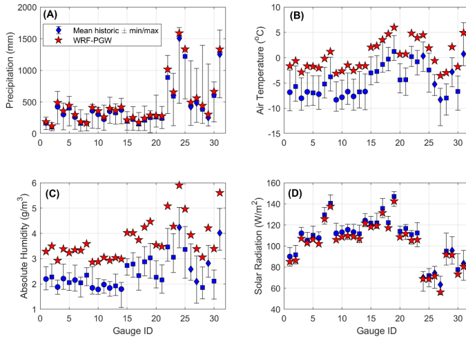
1040 Figure A4: Historic winter climate variability for each predictor used in the stepwise MLR model (Equation 1) for the period between 1045 November and DOS 20 in blue. (A) Precipitation, (B) air temperature, (C) absolute humidity and (D) solar radiation. In red are the perturbed mean climate variables under the RCP8.5 pseudo global warming scenario by the end of the century. This analysis suggests that most of the climate change signal from NoahMP-WRF pseudo global warming is within the observed climate variability, except for air temperature and atmospheric humidity in some watersheds. Blue symbols (circle, square and diamond) associated with historical values represent the mean annual percentage of clear-sky snowmelt days, where sunny sites have >90% clear-sky snowmelt days, partly cloudy have between 70 and 90%, and cloudy have <70%; clear-sky snowmelt days are defined as those with more than 80% of the potential clear-sky solar radiation. We make no inference about the cloudiness condition of snowmelt days under the RCP8.5 pseudo global warming scenario, and thus, we use a five-point star (in red) for the future scenario.
