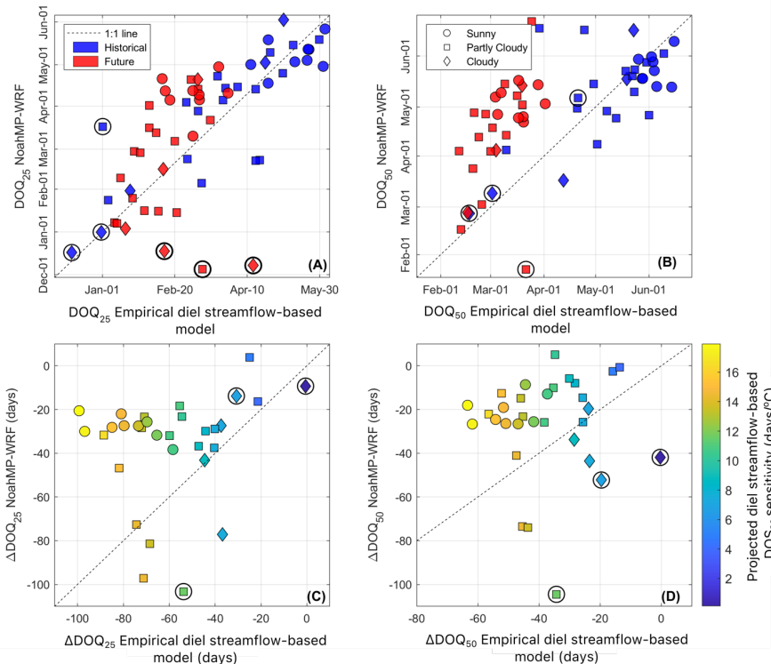
1065 Figure A7: Same as Figure 9 but using streamflow timing metrics from NoahMP-WRF for an RCP8.5 pseudo global warming 1070 scenario, calculated using surface runoff only instead of using surface plus subsurface runoff (as in Figure 6). Note the improved fit 1075 in historical DOQ_{25} ; however, this analysis yields very similar results to those of Figure 6, with NoahMP-WRF streamflow simulations being much less sensitive to climate change than the empirical diel streamflow-based model suggests. (A) and (B) compare historical against projected values between NoahMP-WRF and the empirical diel streamflow-based model. (C) and (D) compare the projected change (future minus historical) between NoahMP-WRF and the diel streamflow-based model, colored by the sensitivity of DOS_{20} to climate change as projected by the empirical diel streamflow-based model (Figure 5b). Symbols surrounded by black circles indicate sites that were excluded from the regression analysis in Figure 3 (rainier sites #24, #25 and #31). Symbols (circle, square and diamond) represent the historical mean annual percentage of clear-sky snowmelt days, where sunny sites have >90% clear-sky snowmelt days, partly cloudy have between 70 and 90%, and cloudy have <70%; clear-sky snowmelt days are defined as those with more than 80% of the potential clear-sky solar radiation. We make no inference about the cloudiness condition of snowmelt days under the RCP8.5 pseudo global warming climate scenario; however, red symbols (upper panels) follow the same symbology for easier interpretation.
