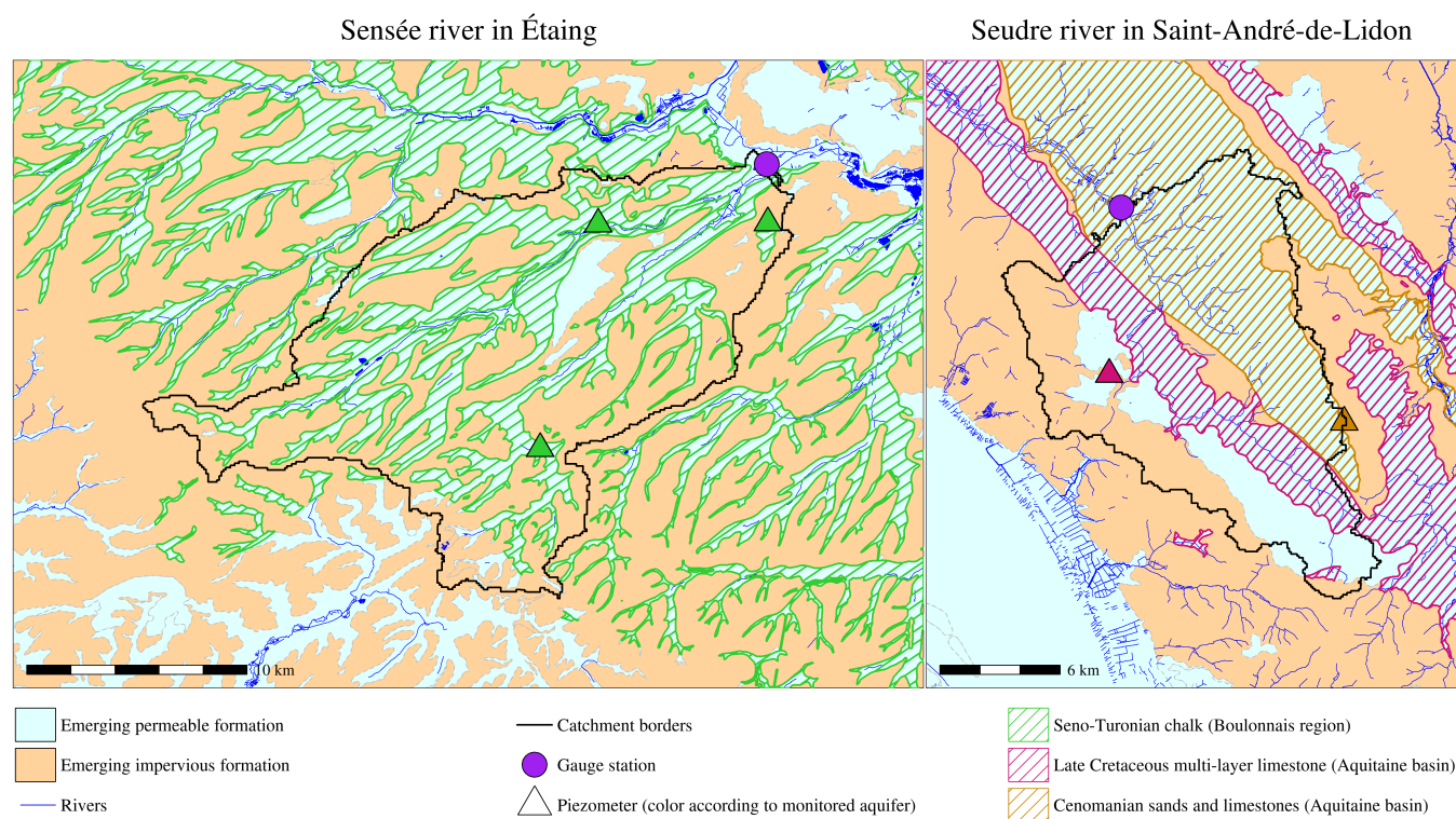
Figure 2. Two examples of hydrogeological maps of catchments used for dataset selection. Their location in the French mainland territory is shown in figure 1.
