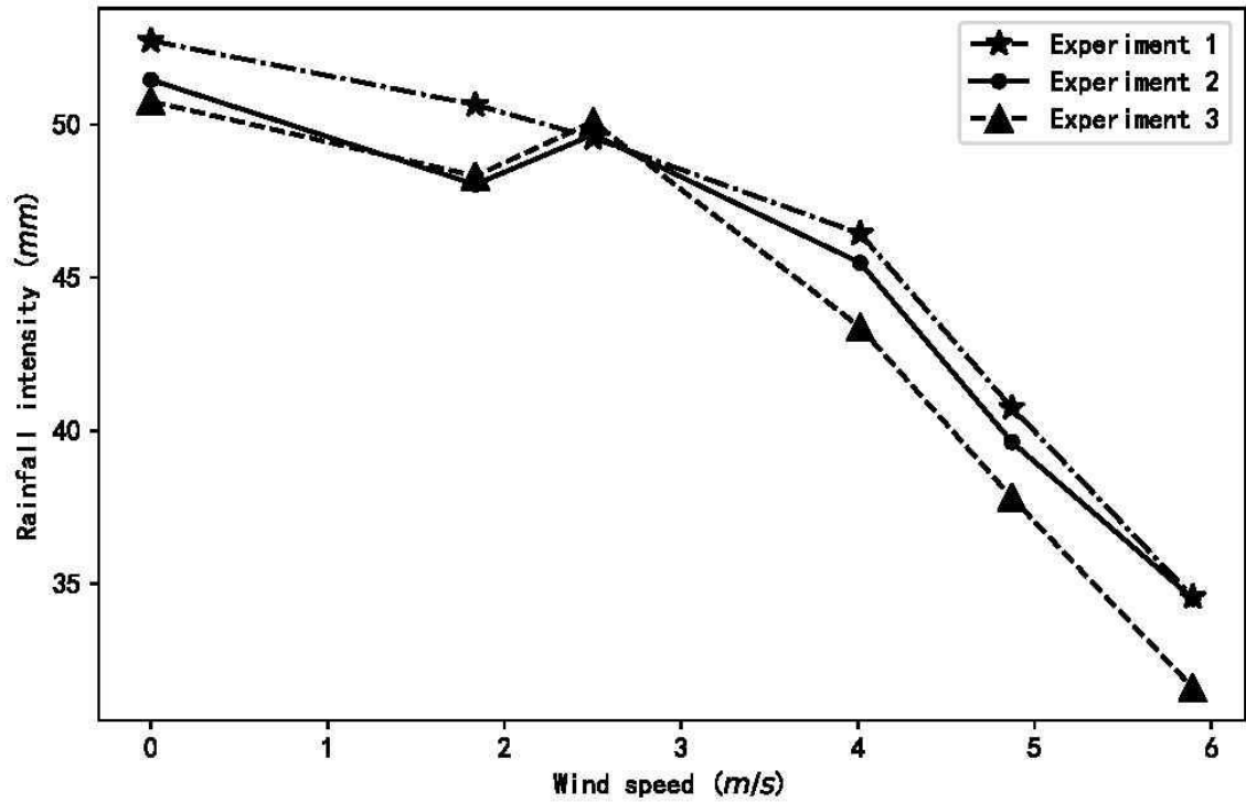
Figure 13: The rainfall intensity atop the scale model under different wind speeds for rainfall 1 of three replicate trials.
