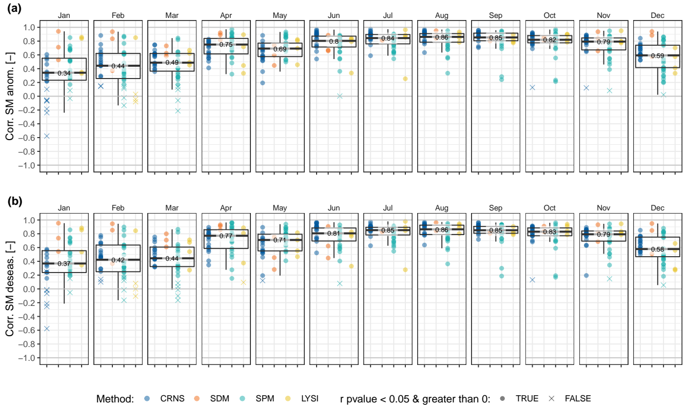
Figure 5. Comparison of the simulated mHM SM (0–25 cm) in the GDM-v2-2021 setup to observed SM anomalies without (a) and with (b) subtraction of the mean seasonal SM cycle for each month depicted with boxplots. SM anomalies are plotted for each location and coloured according to the SM measurement method used. Note that sample sizes between measurement methods differ (CRNS: n=17 , SDM: n=3 , SPM: n=23 , LYSI: n=4 ). Data points that are not both significantly ( p -value < 0.05 ) and positively correlated are marked with x. See Figure A2 for detailed comparisons.
