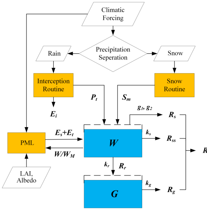
160 Figure 2. The model structure of the DTVGM-PML.
