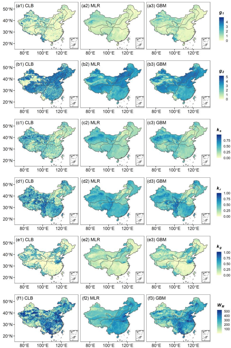
345 | Figure 7. Spatial patterns of model parameters: (a) g_1 , (b) g_2 , (c) k_s , (d) k_r , (e) k_g , (f) W_M , derived from (1) calibration (CLB), (2) multiple linear regression (MLR) and (3) gradient boosting machine (GBM) .
