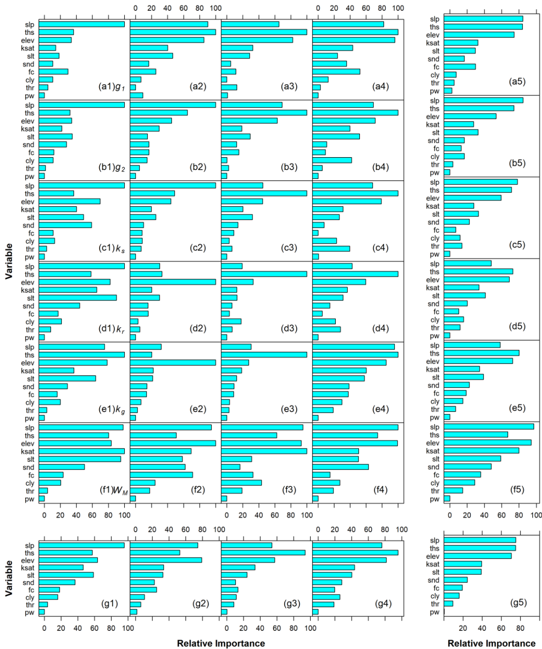
Figure 10. Relative importance of explanatory variables from the gradient boosting machine (GBM) model for (a) g_1 , (b) g_2 , (c) k_s , (d) k_r , (e) k_g , (f) W_M in four climatic zones (1, humid; 2, semi-humid; 3, semi-arid; 4, arid). The mean relative importance over four regions for each parameter is shown in the right column (a5-g5). The mean relative importance over six parameters for each climatic zone is shown in the bottom row (g1-g5). Explanatory variables include elev (Elevation), slp (Slope), snd (Sand content), silt (Silt content), cly (Clay content), fc (Field
