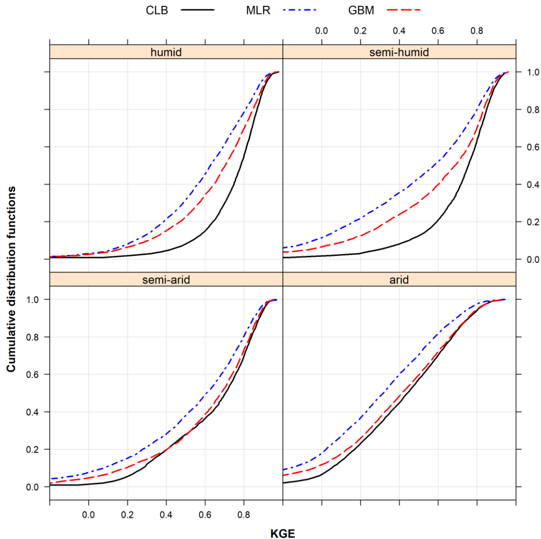
370 Figure 8. Cumulative distribution functions (CDFs) of KGE for runoff simulation based on three parameter sets (black lines for calibration (CLB) , blue lines for multiple linear regression (MLR) , red lines for gradient boosting machine (GBM) ) in the validation period over four climatic zones. KGE denotes the Kling-Gupta efficiency.
