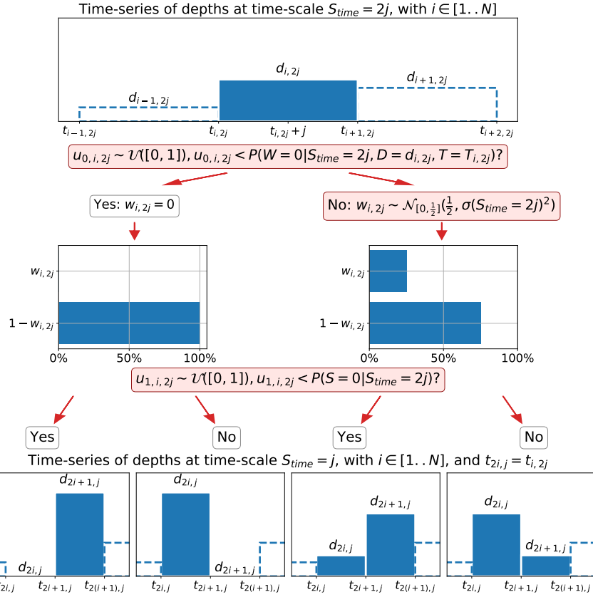
Figure 1. Workflow for downscaling to transfer a depth from time-step T to time-step \frac{T}{2} . The red boxes involve the generation of a random number. The process starts with 1440 minute time-step to reach 5.625 min an interpolation is then done to reach 6 min time-step.
