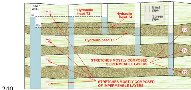
Figure 3. Scheme of the resulting hydraulic head from the existence of permeable stretches with different hydraulic heads. With the plotted dynamic level DL, only T2 contribute water to the well, T4 do not, and T6 collect water from the well.
