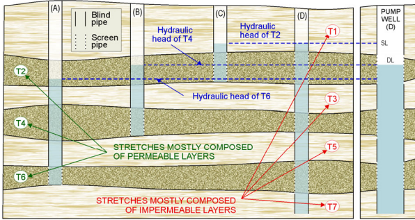
Figure 3. Hypothetical example on the results that would be obtained in a large detrital basin composed of 7 different stretches so that: Permeable stretches T2, T4, and T6 would be hydraulically separated from each other by impermeable stretches T1, T3, T5, and T7; stretches T2, T4, and T6 would have different hydraulic heads, which are drawn in hypothetical wells A, B, C, and D, with different depths and different filtering intervals. Considering the plotted depth and filter intervals of well D, if pumped with the plotted dynamic level DL (coincident with hydraulic head of T4, see the right part of figure), only T2 stretch contributes water to the well, T4 does not, and T6 collects water from the well. Note that the well diameters plotted are not scaled, but highly magnified to enhance the view of the figure.
