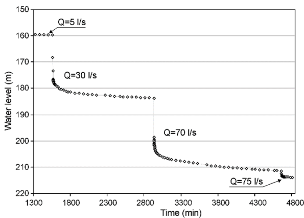
330 Figure 5. Water level versus time during the step-drawdown pumping test in the case study.
