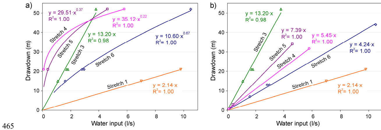
465 Figure 9. Drawdown versus water inputs for different flow stretches in the case study. a) d_N(s) \# q_N(s) with a unique hydraulic head for all the stretches. b) d_N(s) \# q_N(s) with the modified hydraulic heads for each stretch obtained considering that p is at least equal to one in the Rorabough equation).
