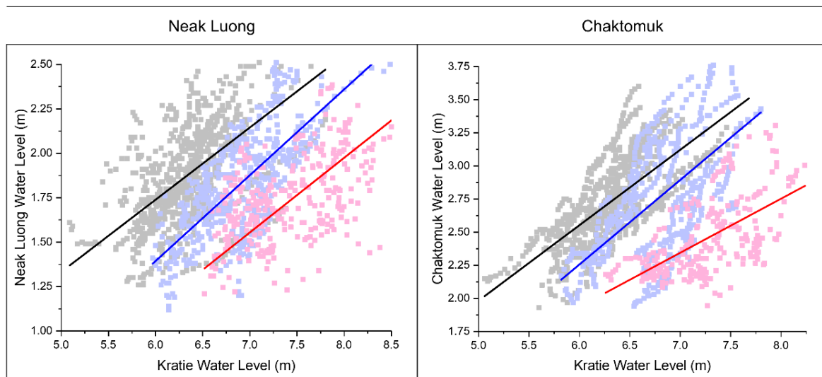
360 Figure 10. Comparison of water levels at Neak Luong/Chaktomuk against water levels at Kratie during February. (Black: 1960-1991; blue: 1992-2009; red: 2010-2019). Given the same water level at Kratie, water levels at Neak Luong/Chaktomuk have been decreasing over time.
