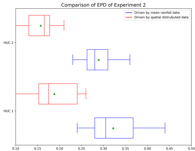
320 Figure 6 Comparison of EPD of Experiment 2 using different types of rainfall data
