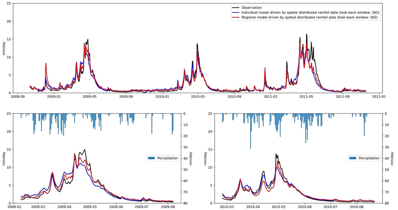
Figure 7 Comparison of performance of Experiment 2 using LSTM as regional model and individual model
