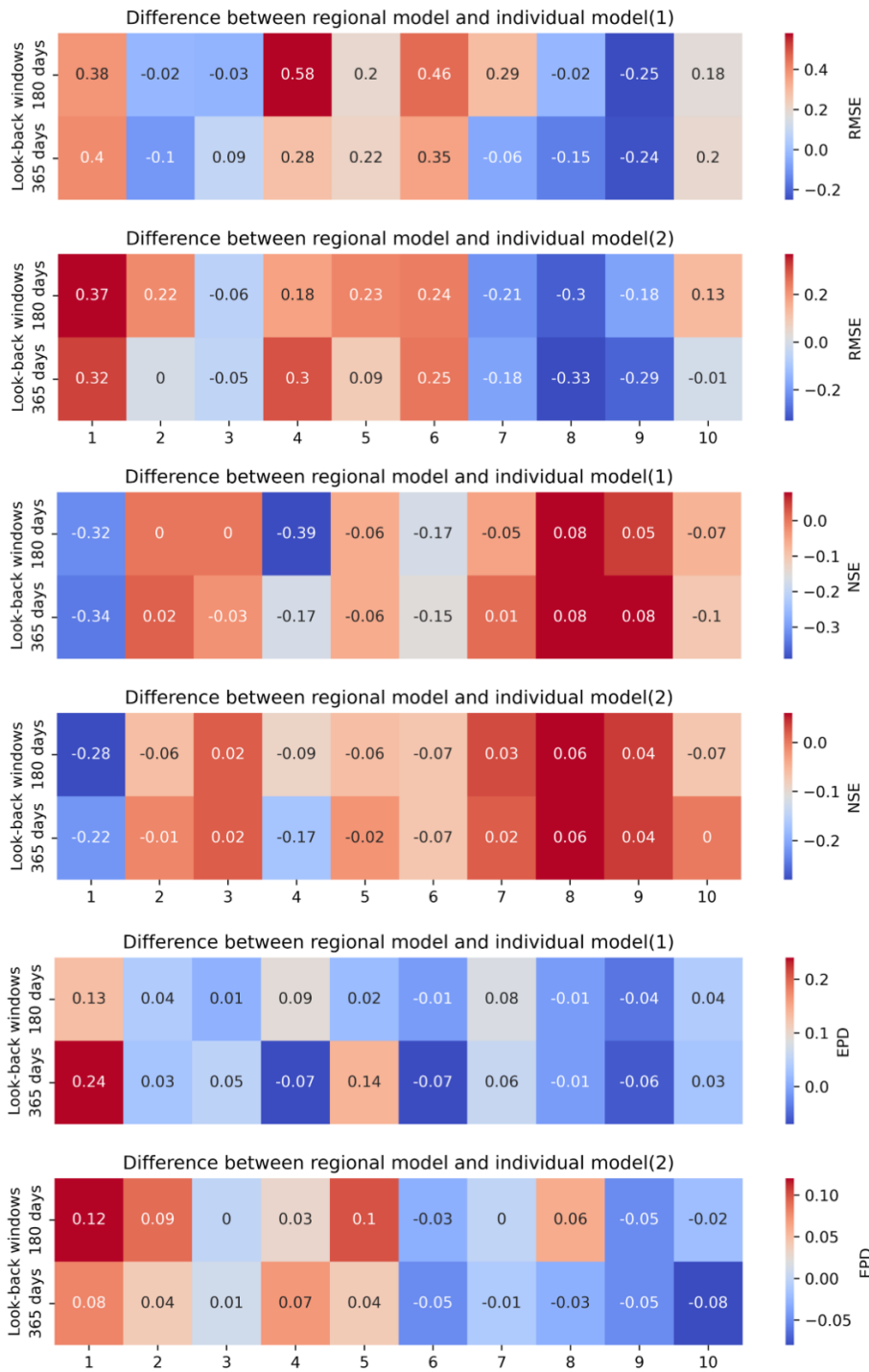
325 Figure 8 Comparison of the performance between using LSTM as a regional model and an individual model: (1) driven by catchment mean rainfall data; (2) driven by spatially distributed rainfall data.
