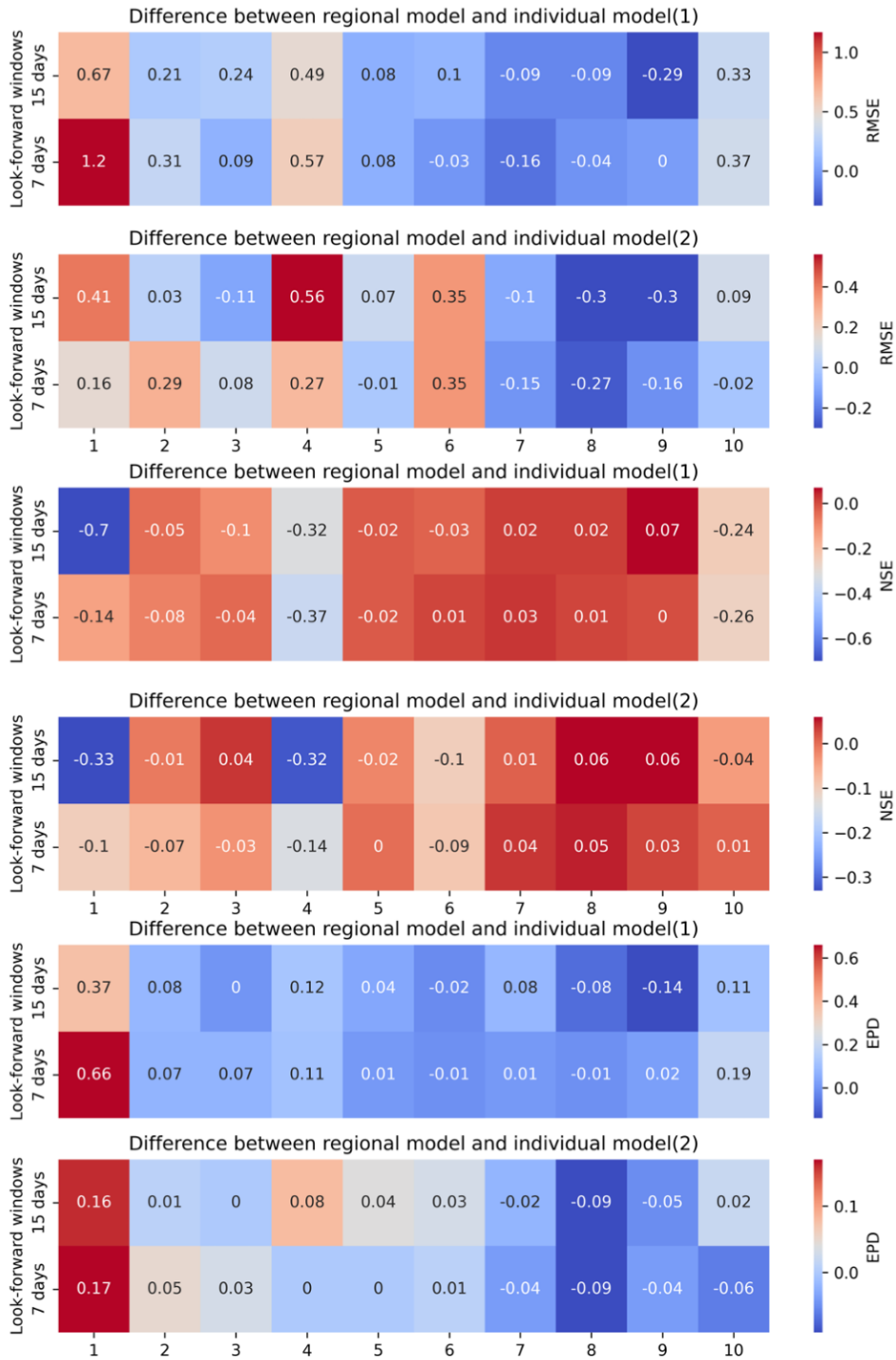
Figure 9 Comparison of the experiment 3 between using LSTM as regional model and individual model: (1) driven by catchment mean rainfall data; (2) driven by spatially distributed rainfall data.
