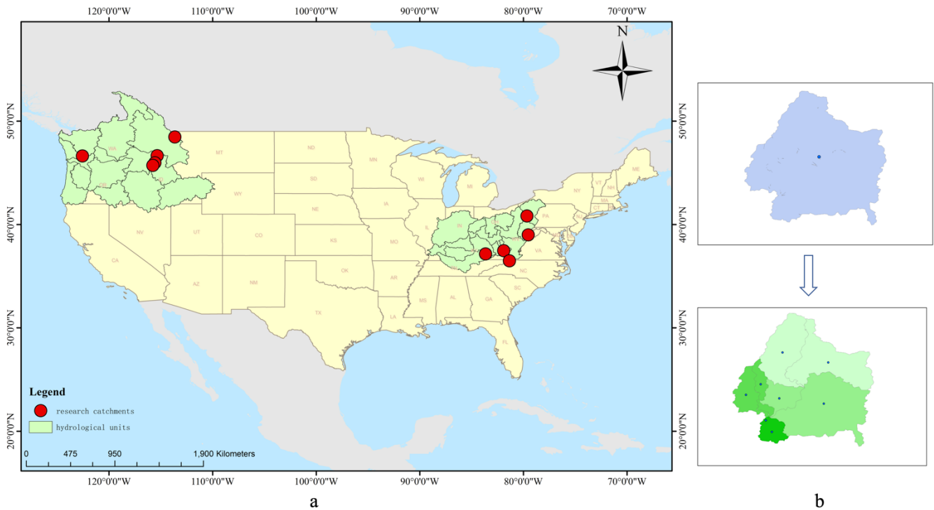
120 Figure1. a: Ten catchments and their locations in the State; b: Examples of spatially distributed rainfall data in this study
