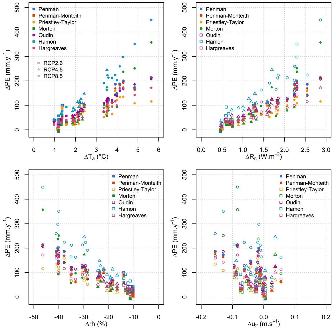
Figure 4. Mean anomalies of annual PE compared to the average anomalies of the climate variables by the end of the century (2070-2099), for air temperature ( T_a , top left), net radiation ( R_n , top right), relative humidity ( rh , bottom left) and wind speed ( u_2 , bottom right). Each symbol represents one combination of RCP/GCM/RCM/PE formulation. Full symbols are used when the climate variable is used in the PE formulation, blank symbols are used when the climate variable is not used in the PE formulation.
