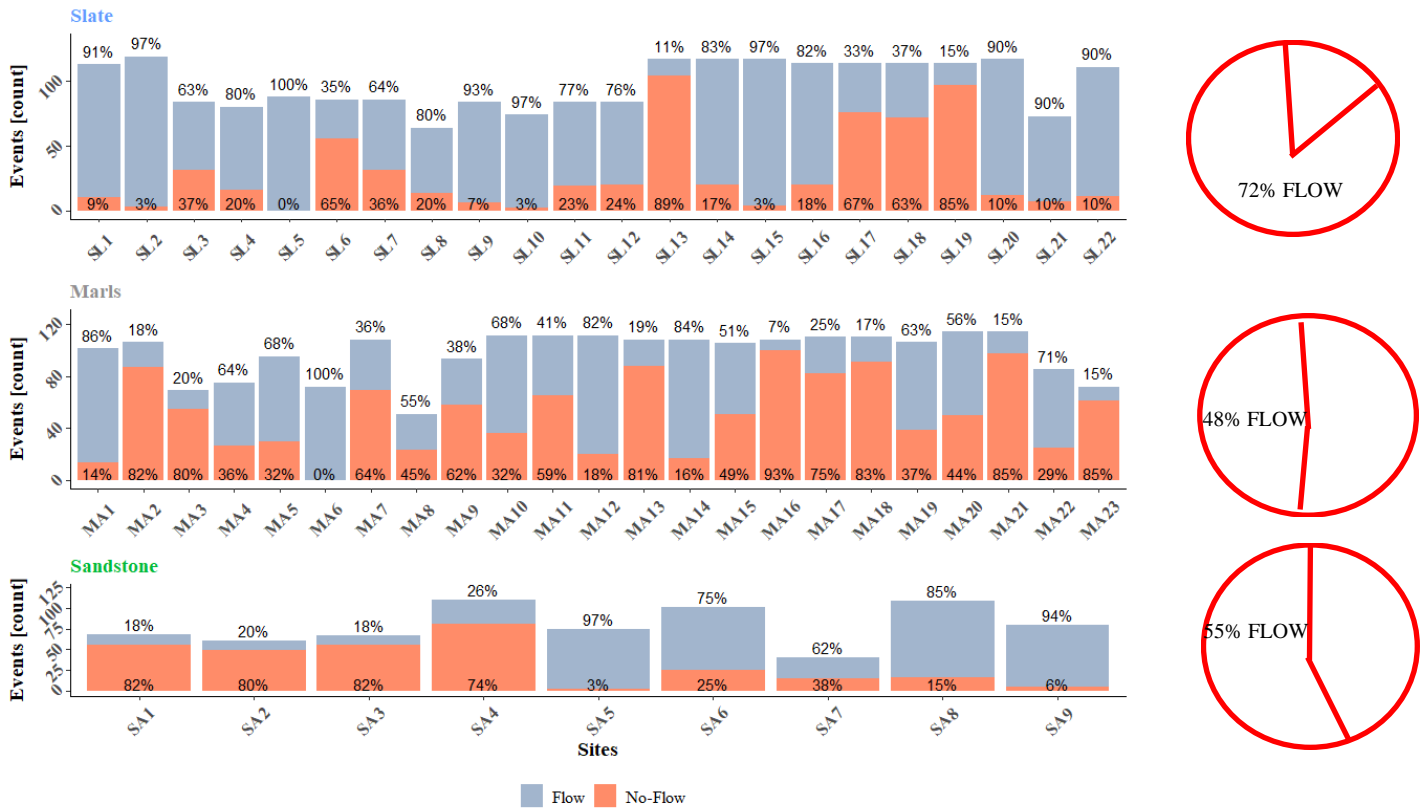
Figure 3: Number of precipitation events having either flow or no-flow reactions in the geologies slate, marls, and sandstone.
