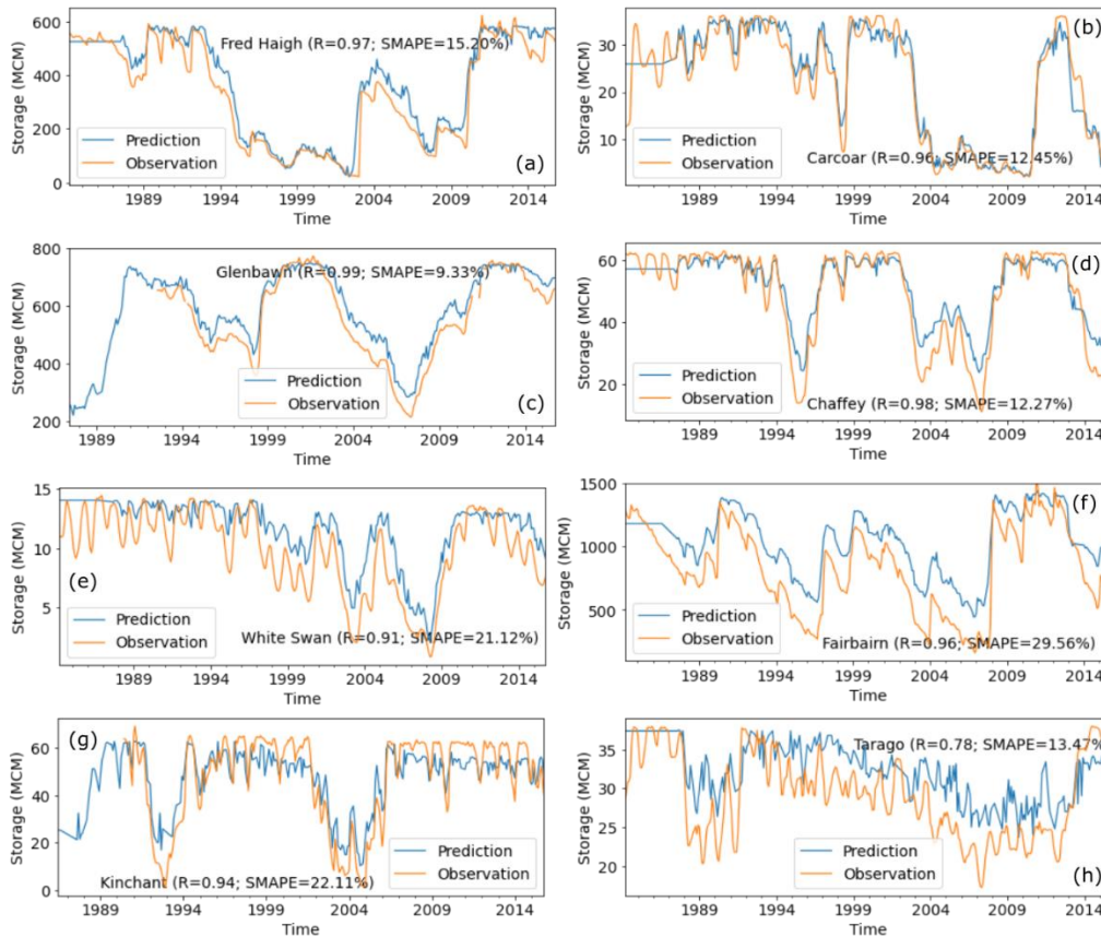
235 Figure 2 Validation of monthly reservoir storage time series reconstruction against in situ storage data, showing (a, b) robust, (c, d) typical and (e, f) poor results.
