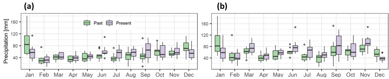
Figure 3: Monthly mean precipitation averaged over the two periods: past (1965-1975) and present (2008-2018). (a) AGRB (b) PGRB.
