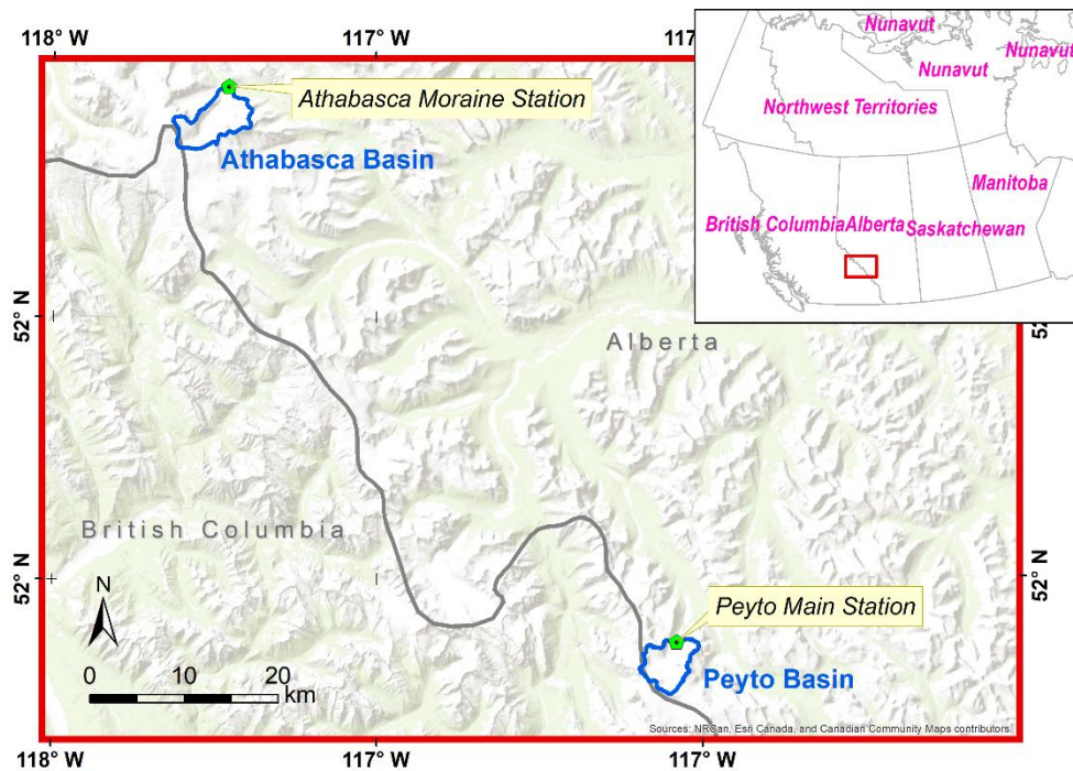
5 Figure 1: Location map of Peyto and Athabasca glacier research basins. Gray line is the border between two provinces, blue polygons are basin boundaries, and green pentagons are meteorological stations.
