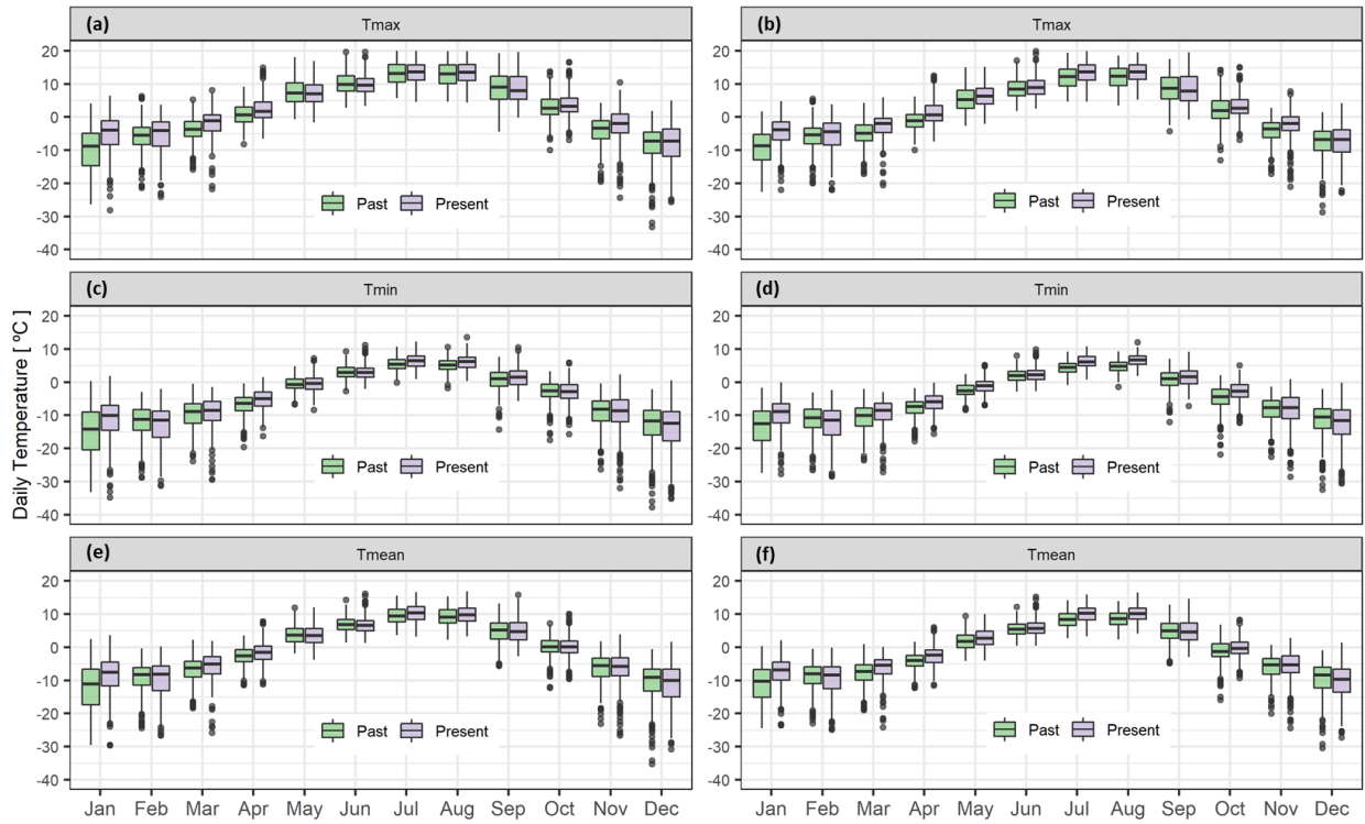
Figure 2: Monthly means of daily maximum (a, b), minimum (c, d) and mean (e, f) temperature comparison between two periods: past (1965-1975) and present (2008-2018). (a, c, and e) AGRB (b, d, f) PGRB.
