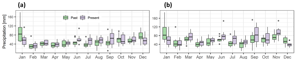
5 Figure 3: Monthly mean precipitation averaged over the two periods: past (1965-1975) and present (2008-2018). (a) AGRB (b) PGRB.
