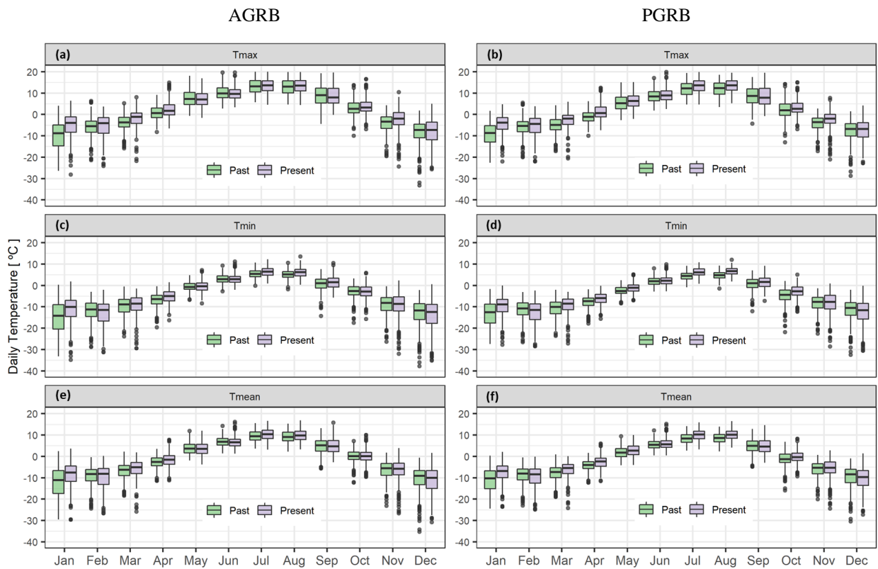
Figure 2: Monthly means of daily maximum (a, b), minimum (c, d) and mean (e, f) temperature comparison between two periods: past (1965-1975) and present (2008-2018). (a, c, and e) AGRB (b, d, f) PGRB.
