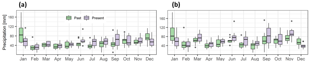
5 Figure 3: Monthly mean precipitation averaged over the two periods: past (1965-1975) and present (2008-2018). (a) AGRB (b) PGRB.
