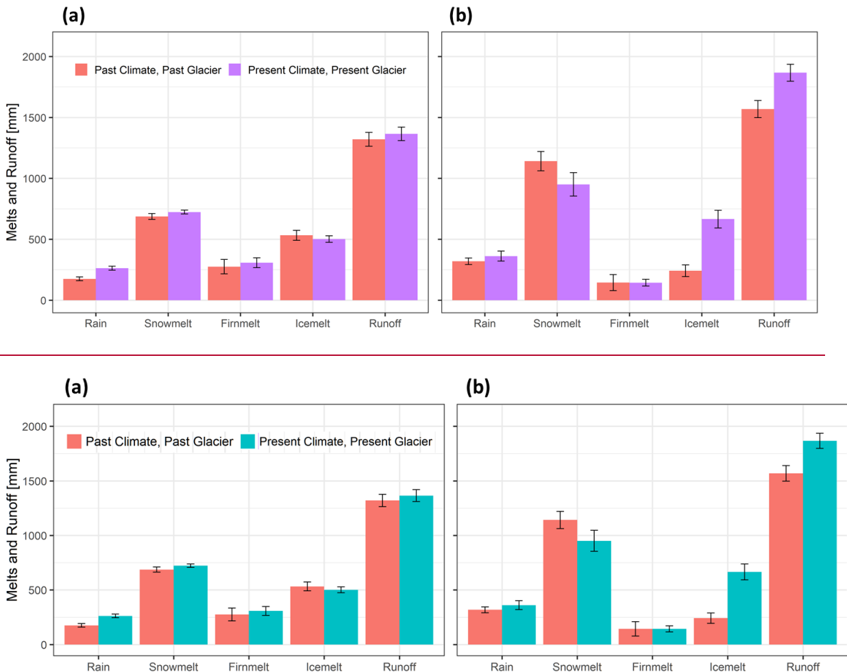
Figure 7: Mean annual melt, rainfall-runoff and basin runoff for the past and present glacier configuration and climate scenarios. Error bars show the annual variability, defined as the standard error between years. (a) AGRB (b) PGRB.
