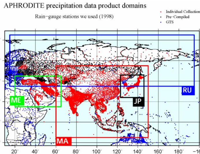
Figure 2. APHRODITE data ( http://aphrodite.st.hirosaki-u.ac.jp/products.html )
