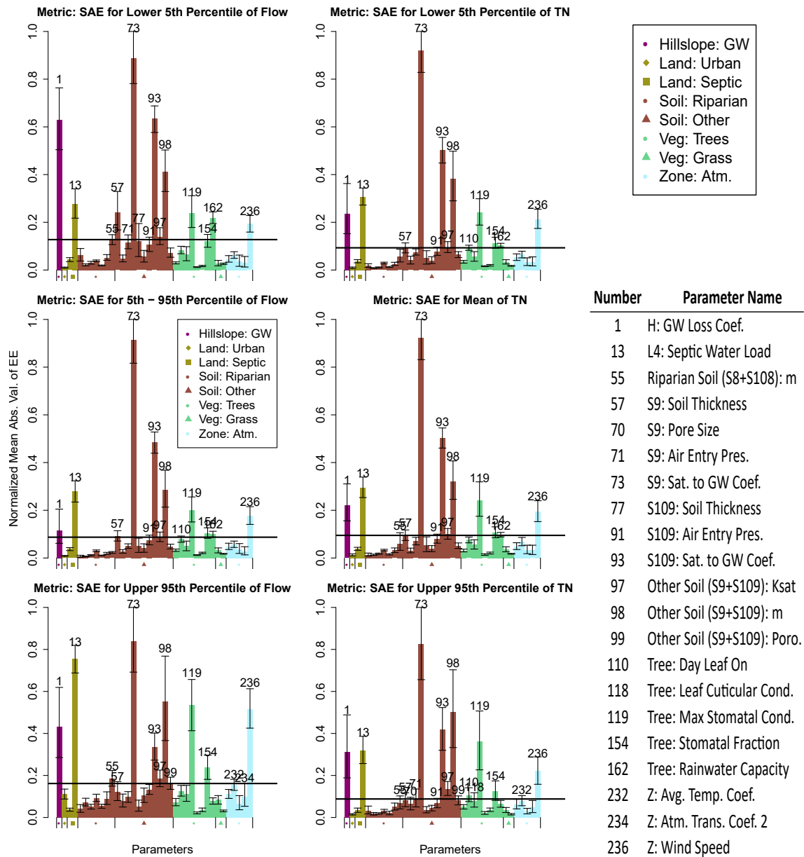
Figure 3. Mean absolute value of elementary effects for RHESSys model parameters evaluated for the six decision-relevant sensitivity metrics at the basin outlet . Effects-EEs are normalized such that the maximum error bar value is equal to 1 on each plot. Only parameters that would be selected by any metric presented in Table 1 are plotted in this figure . Colors indicate to which RHESSys category parameters belong, and symbols distinguish types within each category. Bootstrapped error bars extend from the 5 th to 95 th percentiles. Numbers above the error bars indicate the order along the x-axis for those -parameters greater than the 10% cutoff (black horizontal line in each plot). These The numbered parameters are displayed in the accompanying table. Supplementary tables contain the data plotted in this figure (item S1). Abbreviations: GW - groundwater, Ksat - saturated hydraulic conductivity (cond.), m - describes cond. decay with sat., poro. - porosity, trans. - transmissivity.
