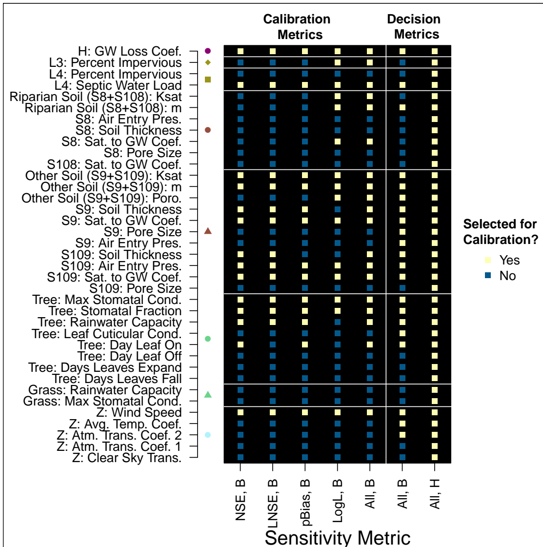
Figure 7. Mean absolute value of elementary effects Indicators for RHESSys model parameters evaluated whether or not a parameter would be selected for calibration for each of the four calibration-relevant sensitivity metrics, and separately aggregated over all calibration-relevant and decision-relevant sensitivity metrics. The style matches B and H in the x-axis labels indicate basin outlet or hillslope outlet. Vertical white lines divide the calibration and decision-relevant sensitivity metric results. Other styles match Figure 34B.
