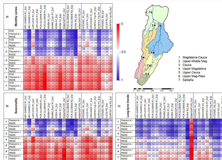
Figure 11. Summary figure of the models performance respect to GRACE data. Statisticians of KGE, Pearson's r, and RMSE were rescaled between 0 and 1, with 0 being the worst performance among the models and 1 being the best performance. The evaluation for the monthly time series is presented in a), in b) the evaluation for the seasonality, and in c) for the long-term trends.
