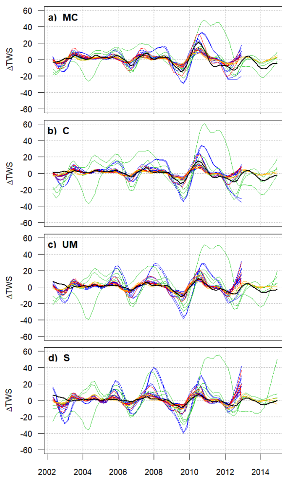
Figure 10. Long-term trends time series for the models and GRACE for a) MC, b) Cauca, c) UM, and d) Saldaña basins. The black line indicates the GRACE JPL, the blue and green lines the GHM WRR1 and WRR2 respectively, the red lines the LSM WRR1 and the yellow lines the LSM WRR2.
