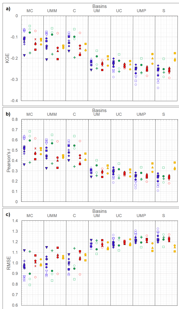
Figure 4. Performance statistics between GRACE and the GHM (blue and green points for WRR1 and WRR2 respectively) and LSM (red and yellow points for WRR1 and WRR2) at different scales. In a) the KGE index, b) Pearson's r , and c) the RMSE. The basins are ordered by size (largest to the left), and the data is standardized and normalized.
