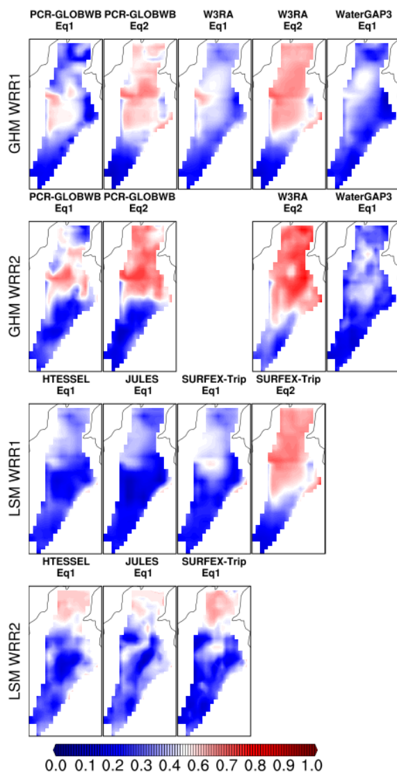
Figure 5. GRACE JPL vs Models correlation maps for those that are available both in WRR1 and WRR2 for Eq1 and Eq2.
