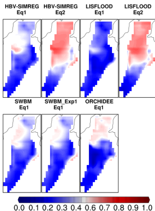
Figure 6. GRACE JPL vs Models correlation maps for those that are available only in WRR1 for Eq1 and Eq2.
