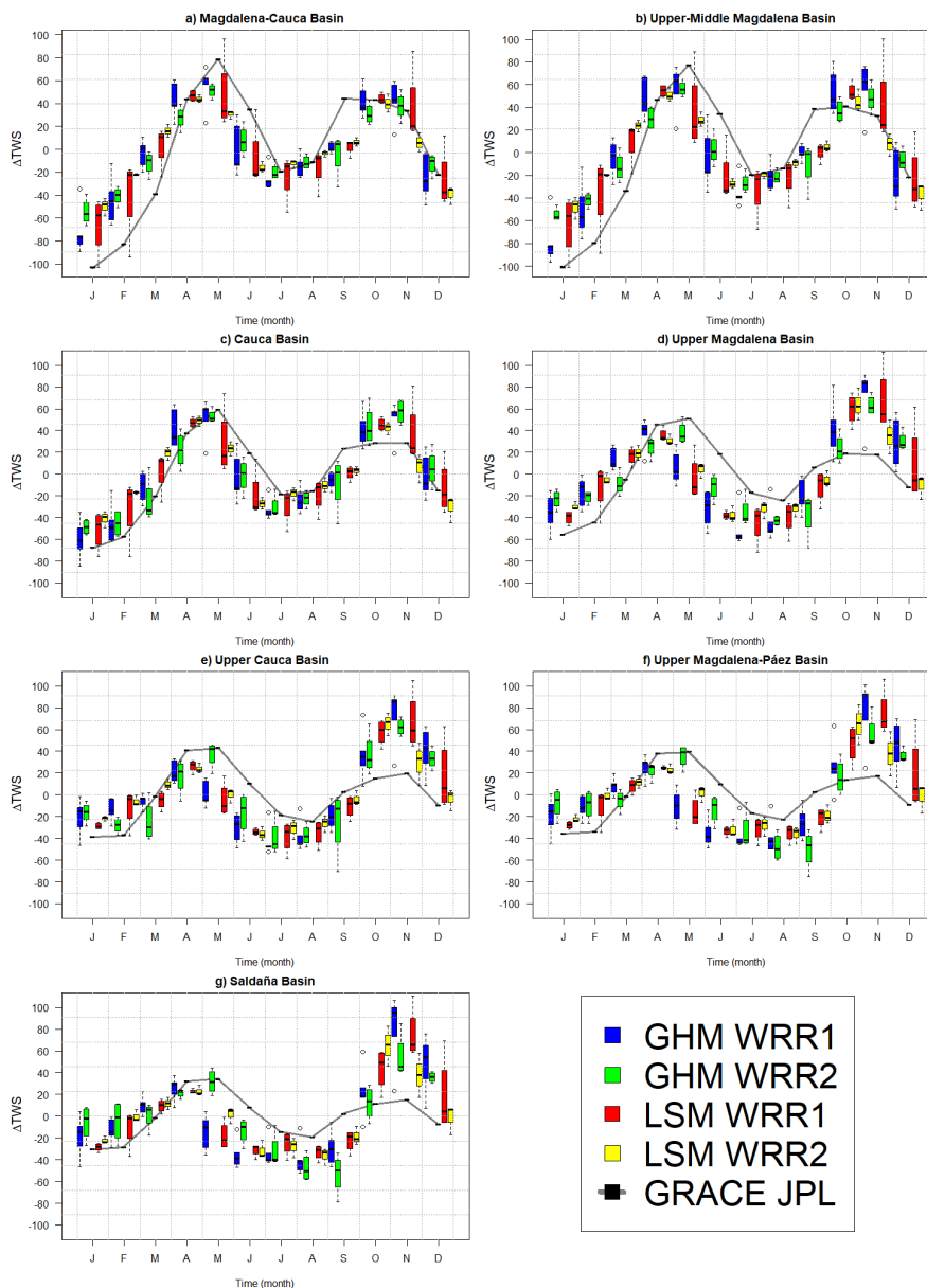
Figure 8. Comparative boxplots between the climatology of GHM and LSM, and GRACE JPL for each subbasin.
