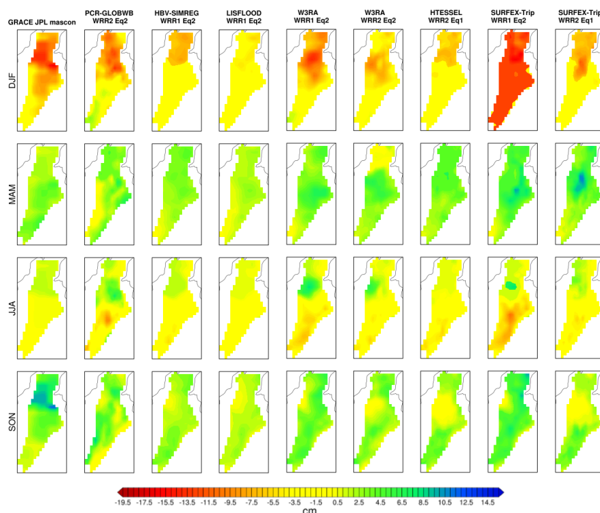
Figure 9. Seasonal maps for GRACE JPL, GHM, and LSM.
