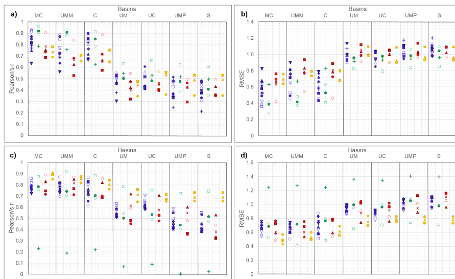
Figure 7. Performance statistics for the seasonality (a–b) and long-term trends (c–d) of GRACE and the GHM (blue and green points for WRR1 and WRR2 respectively) and LSM (red and yellow points for WRR1 and WRR2) at different scales. In a) and c) the Pearson's r coefficient and in b) and d) the RMSE.
