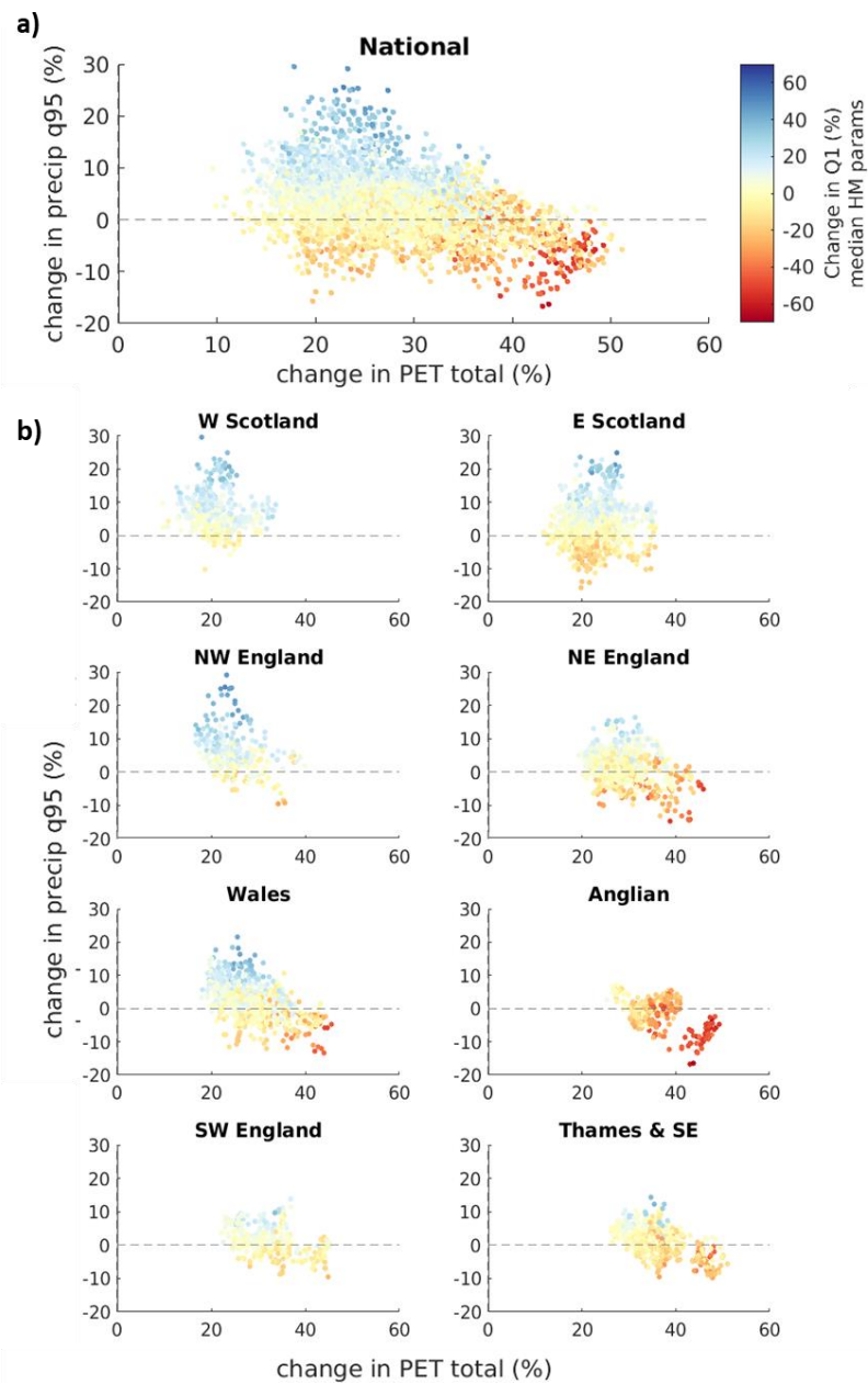
Figure 98: Relationship between changing climate and changing high flows (Q1), shown for all catchments nationally (a) and by region (b). Plots show climatic changes from all RCMs, coloured by the median change in Q1 flows from the ensemble of hydrological model parameter sets. Regions which are shown together, exhibited similar patterns.
